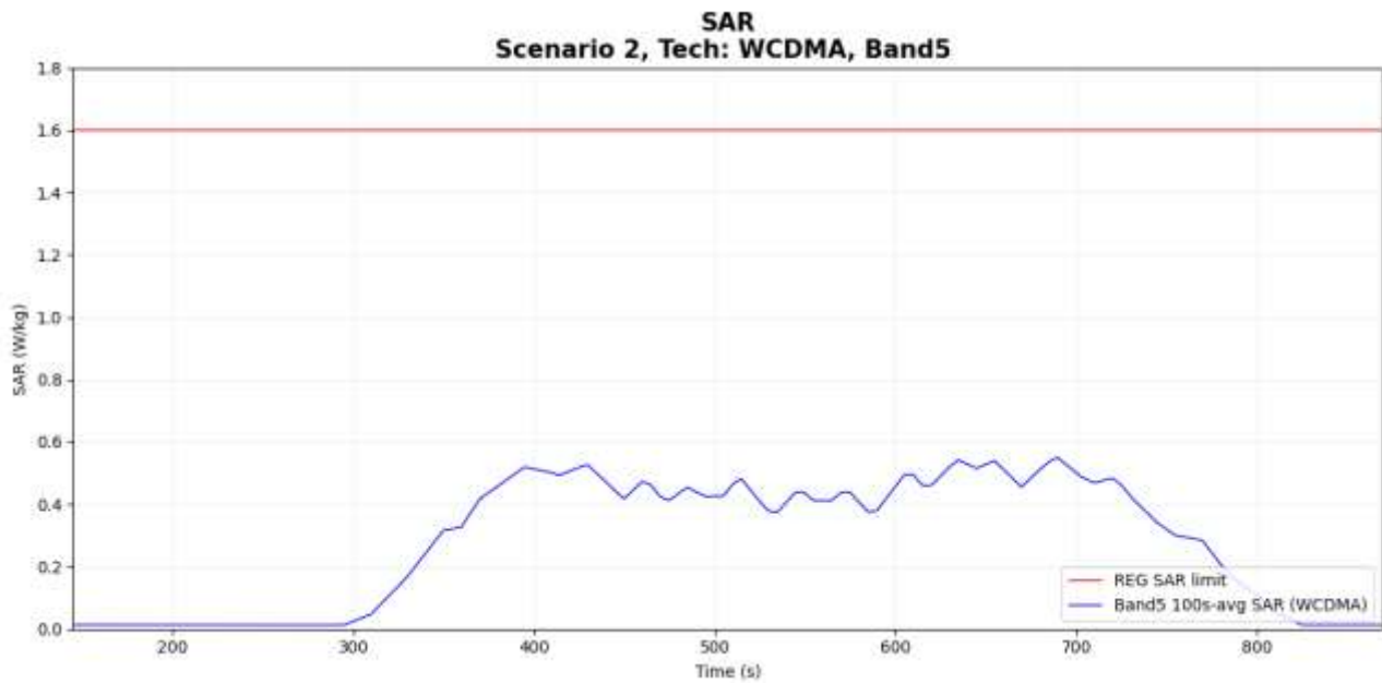
Figure 7-7 Time-averaged SAR
