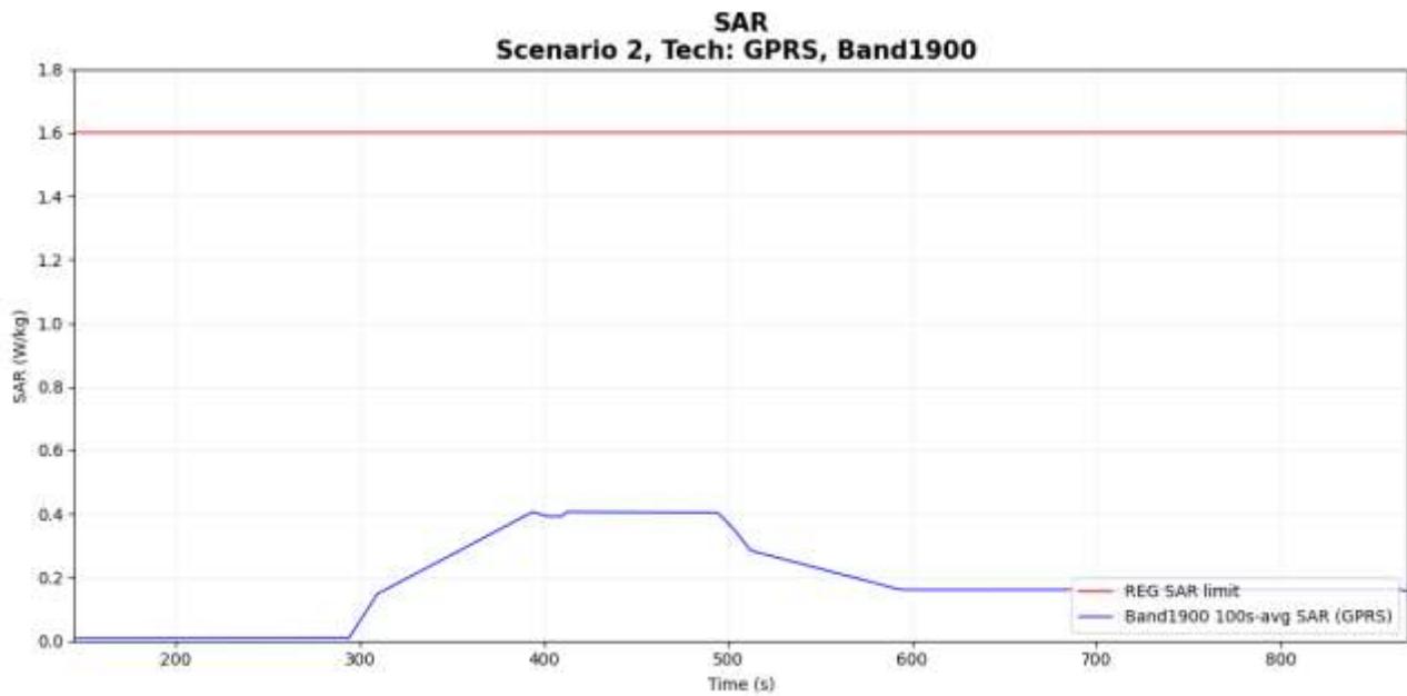
Figure 7-4 Time-averaged SAR
