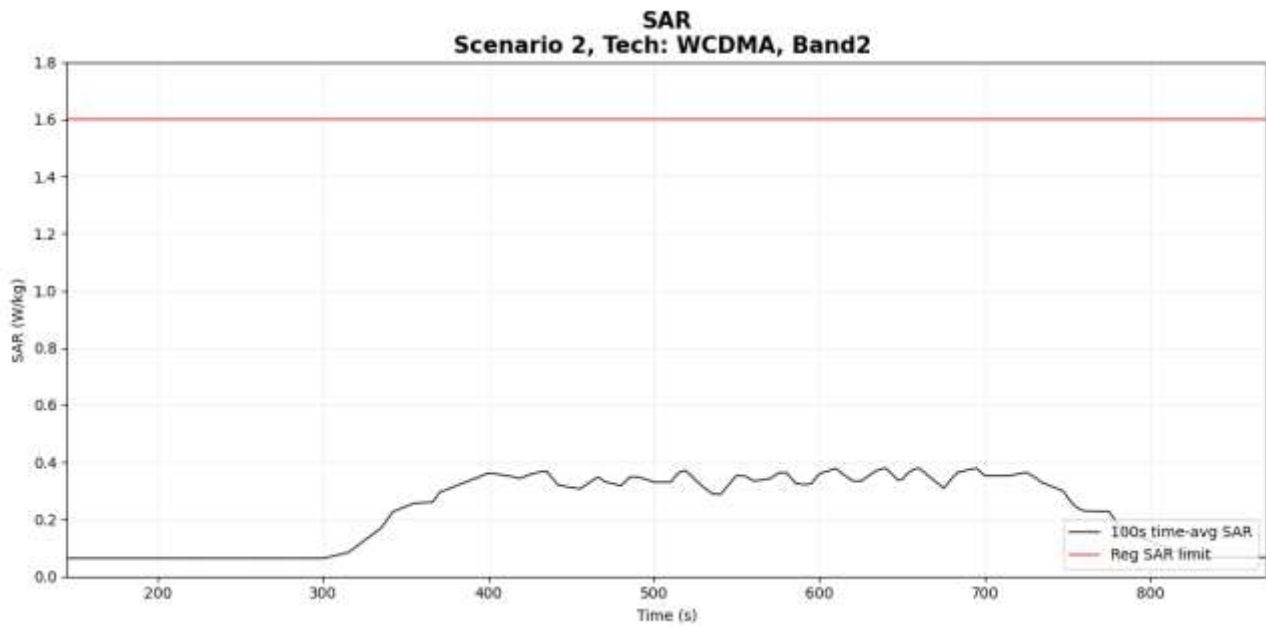
Figure 6- 12 Time-averaged SAR
