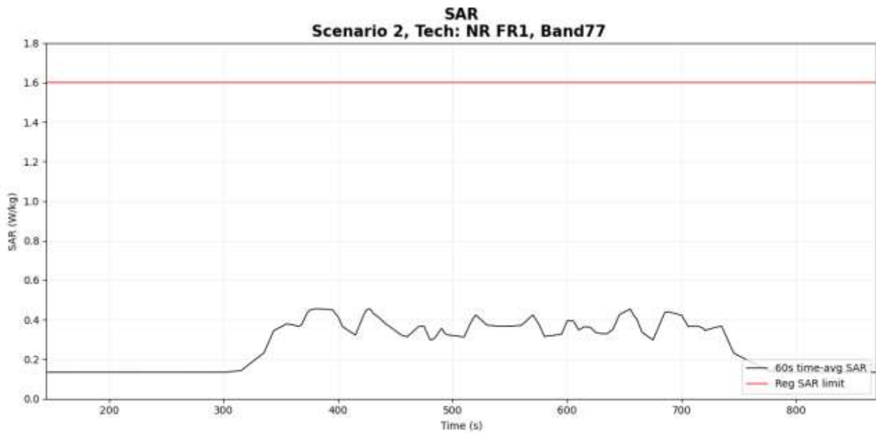
Figure 6- 20 Time-averaged SAR
