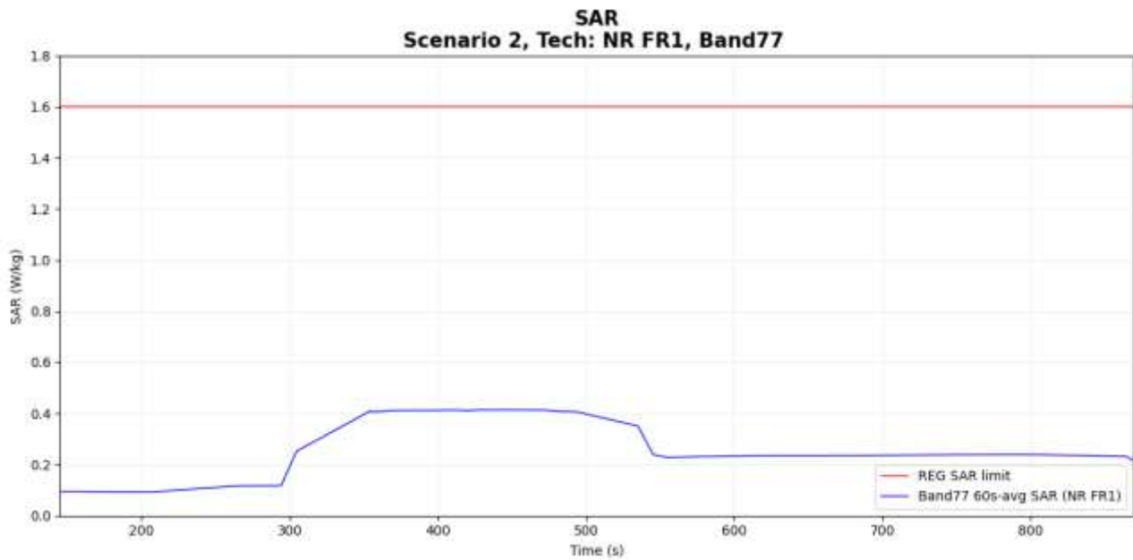
Figure 7-16 Time-averaged SAR
