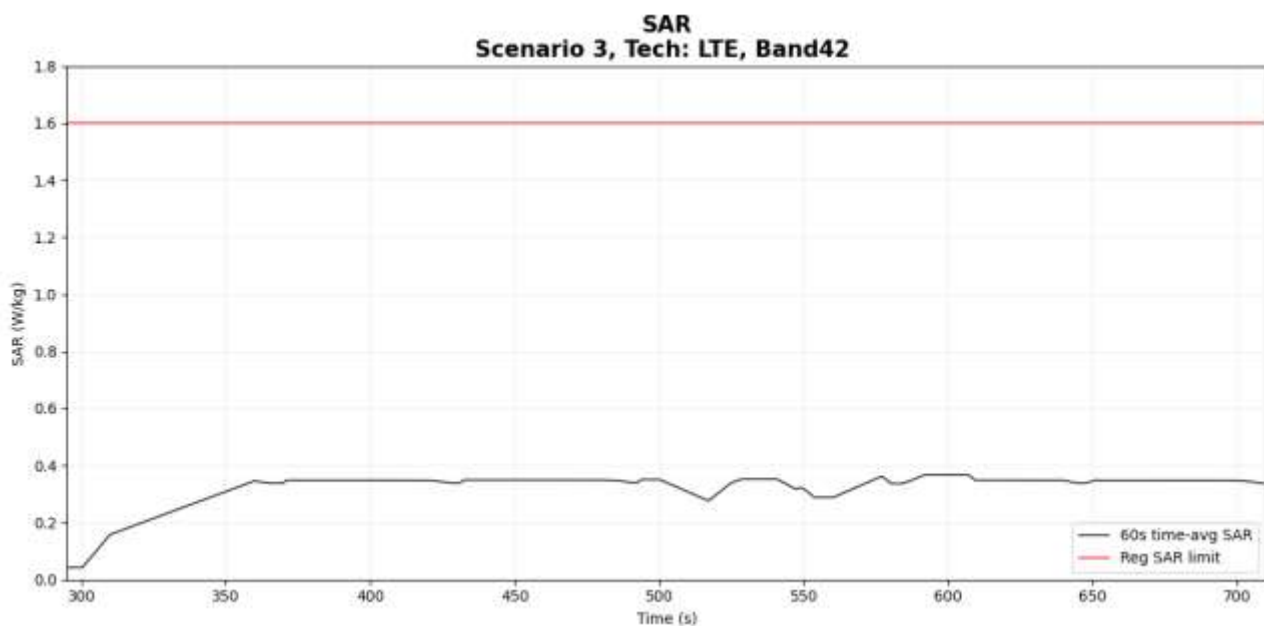
Figure 6- 21 Time-averaged SAR
