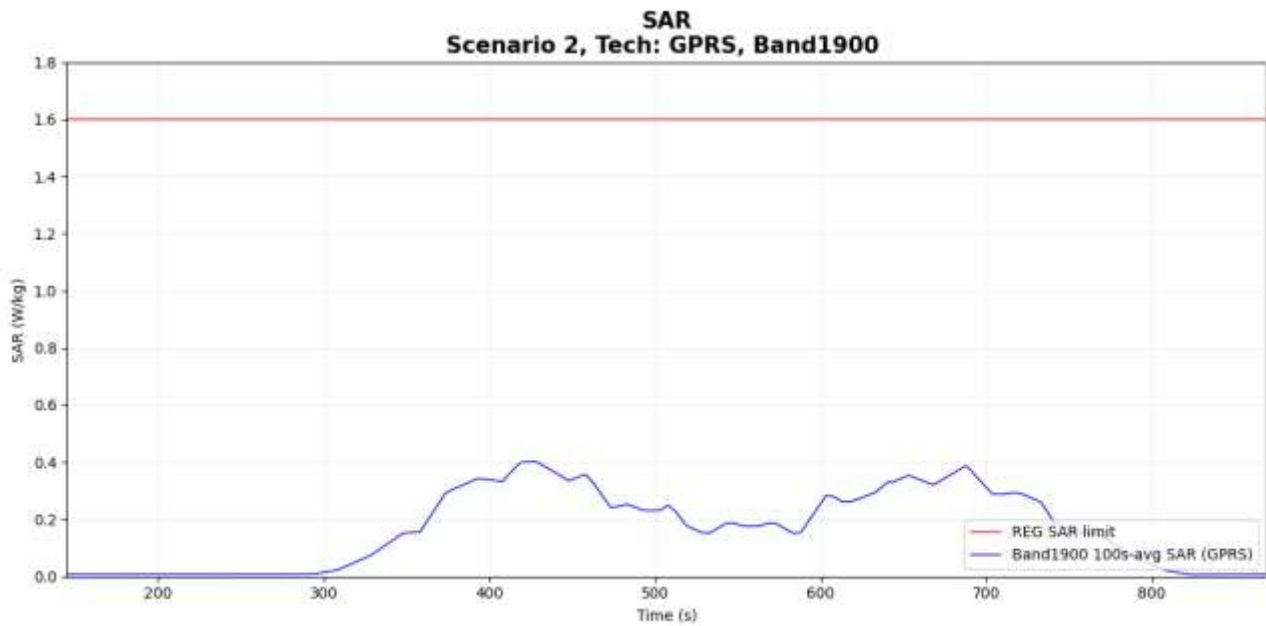
Figure 7-5 Time-averaged SAR
