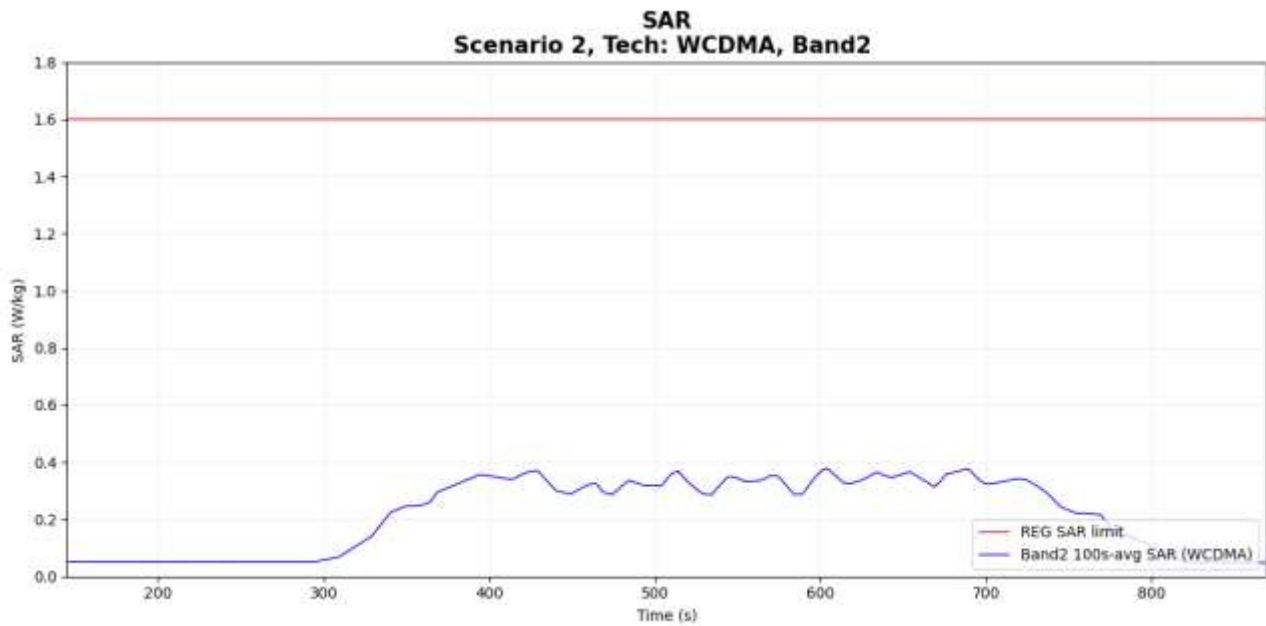
Figure 7-9 Time-averaged SAR
