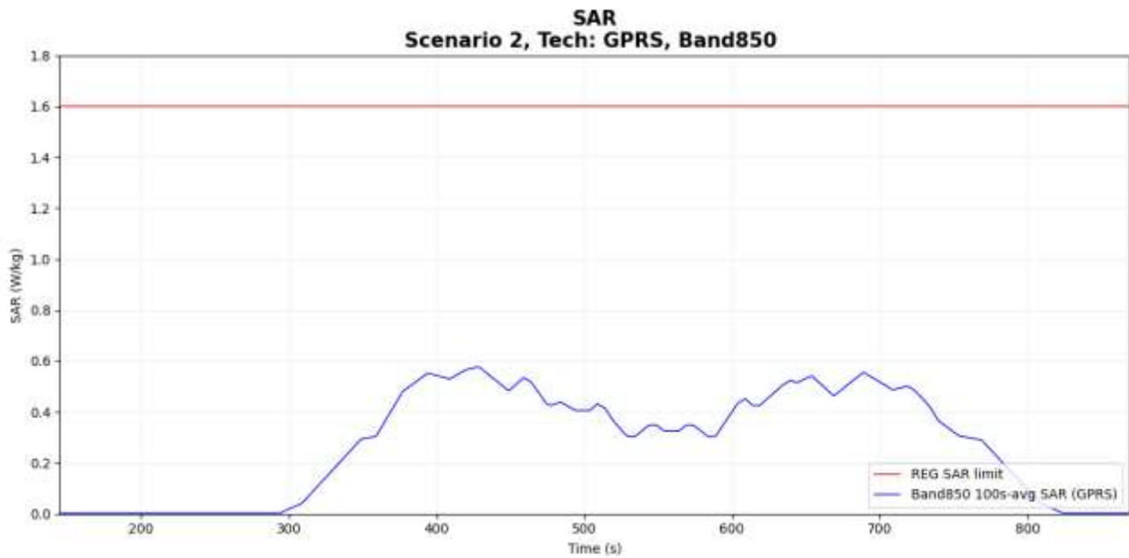
Figure 7-3 Time-averaged SAR
