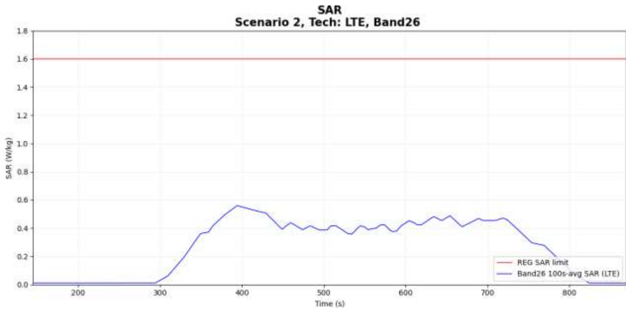
Figure 7-11 Time-averaged SAR
