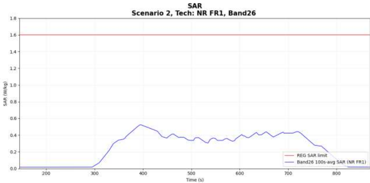
Figure 7-15 Time-averaged SAR
