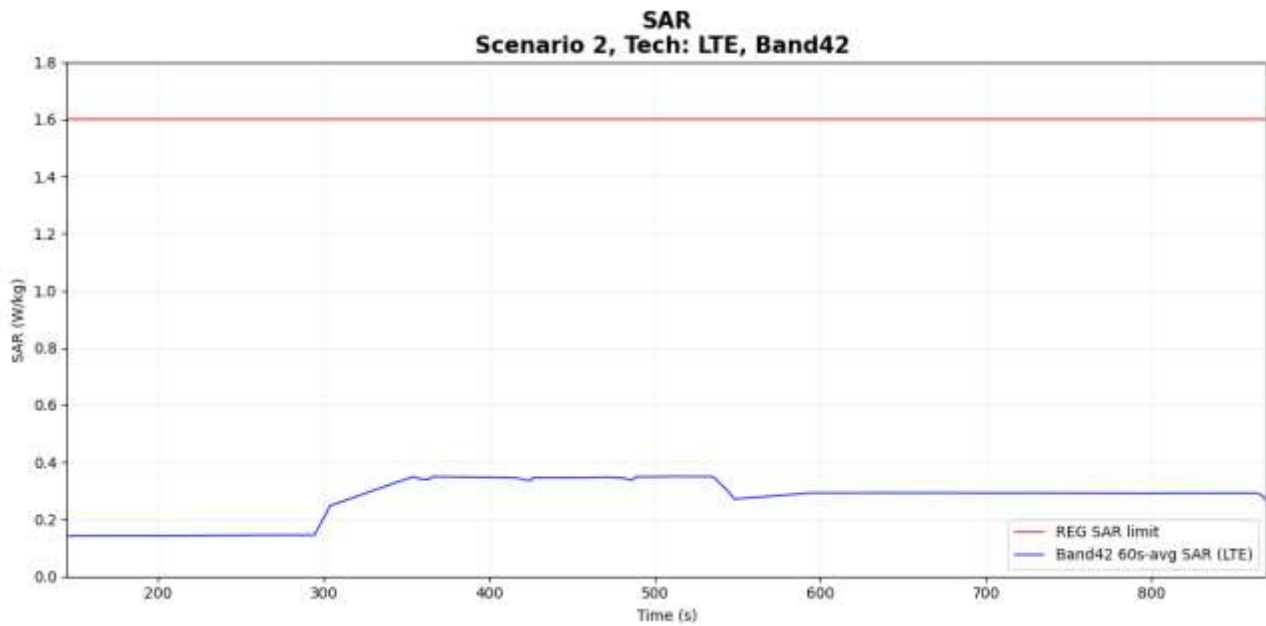
Figure 7-12 Time-averaged SAR
