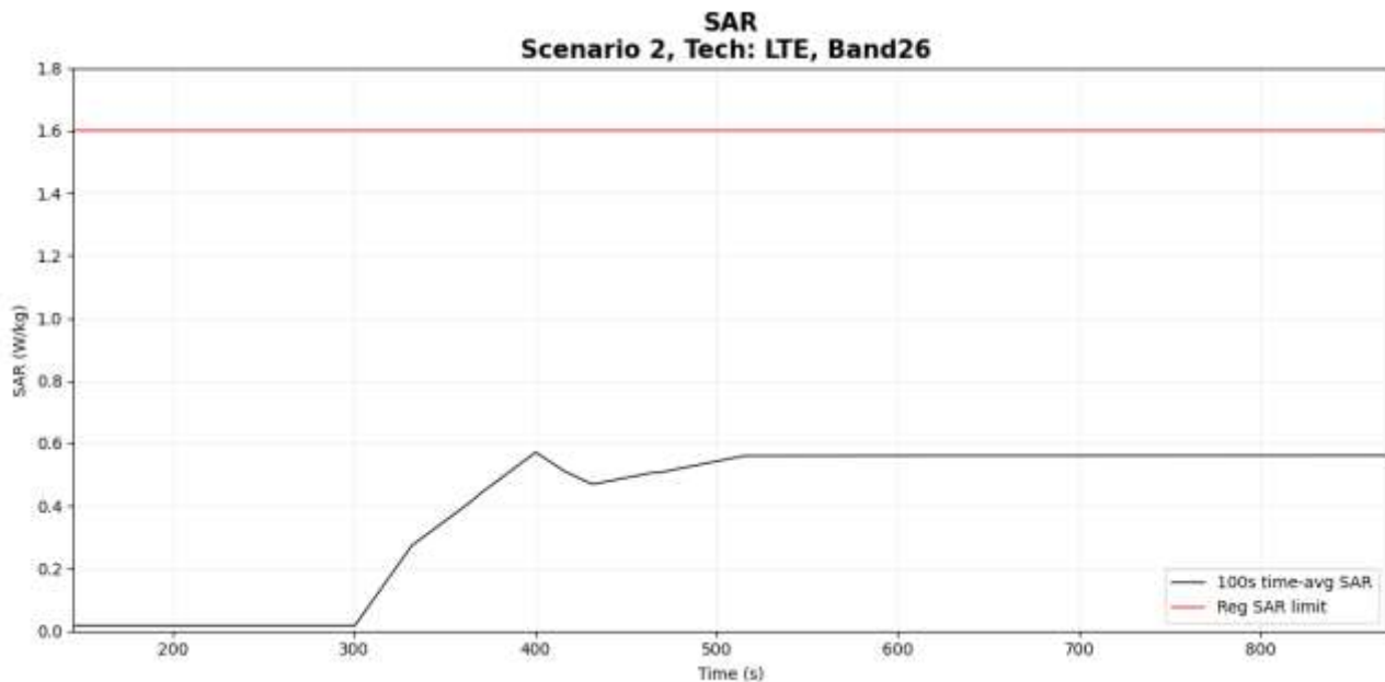
Figure 6- 13 Time-averaged SAR
