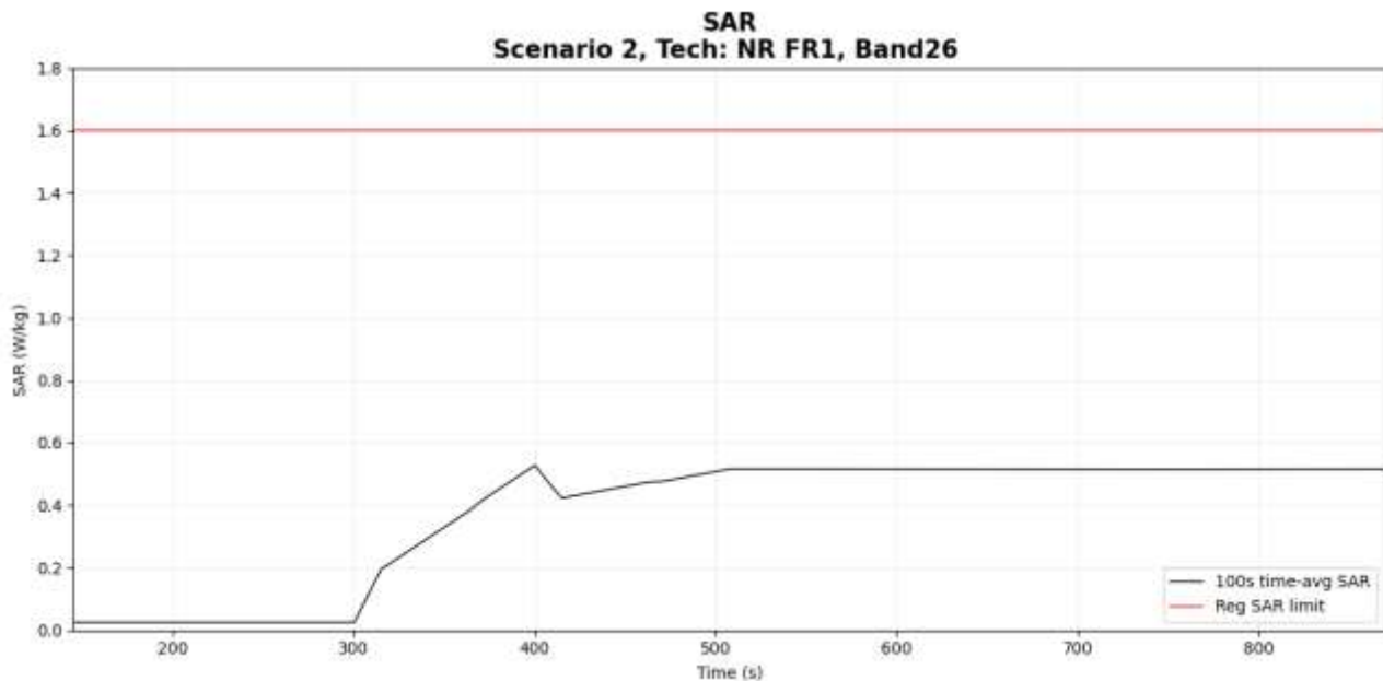
Figure 6- 17 Time-averaged SAR
