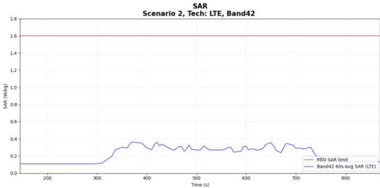
Figure 7-13 Time-averaged SAR
