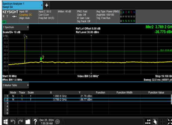
N2(20M)_DFT-s- OFDM_BPSK_Edge_1RB_Left_High_CH
