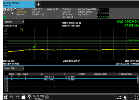
N2(20M)_DFT-s- OFDM_QPSK_Edge_1RB_Left_High_CH
