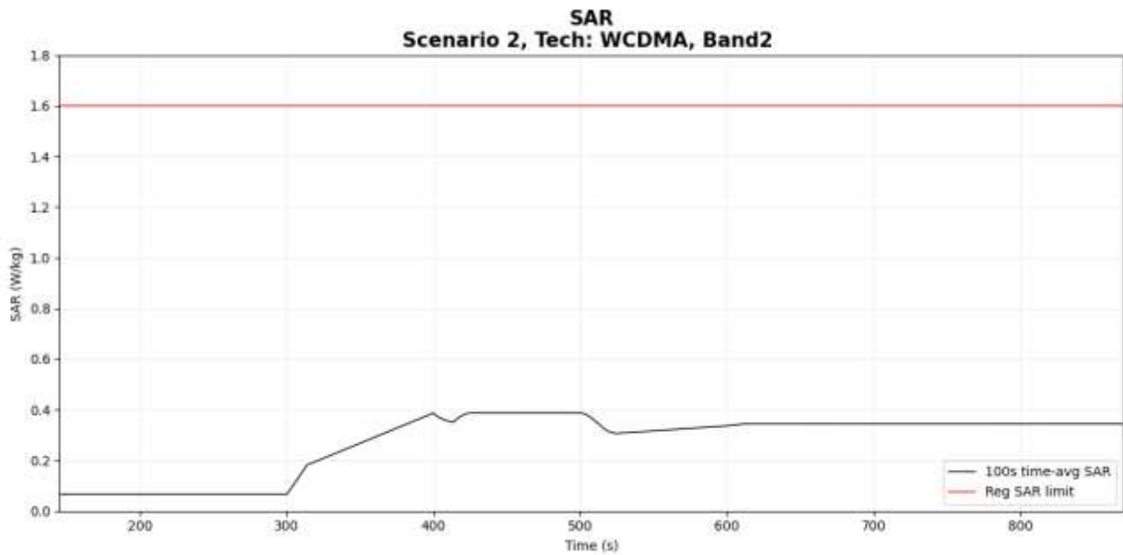
Figure 6- 11 Time-averaged SAR
