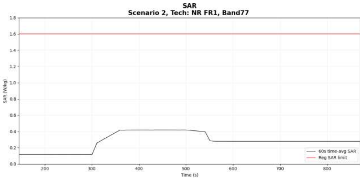
Figure 6- 19 Time-averaged SAR
