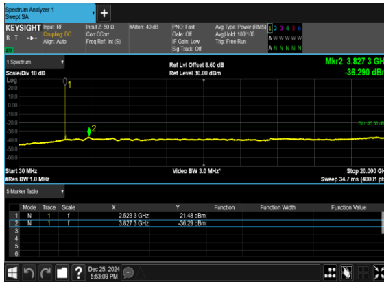
B2_N7(25M)_DFT-s- OFDM_BPSK_Edge_1RB_Left_Mid_CH
