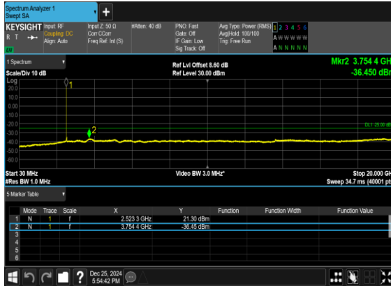
B2_N7(25M)_DFT-s- OFDM_QPSK_Edge_1RB_Left_Mid_CH
