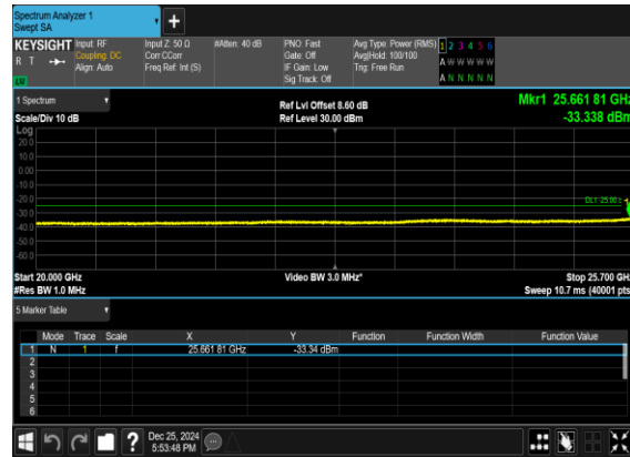
B2_N7(25M)_DFT-s- OFDM_BPSK_Edge_1RB_Left_Mid_CH
