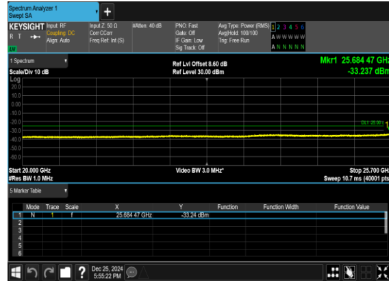
B2_N7(25M)_DFT-s- OFDM_QPSK_Edge_1RB_Left_Mid_CH
