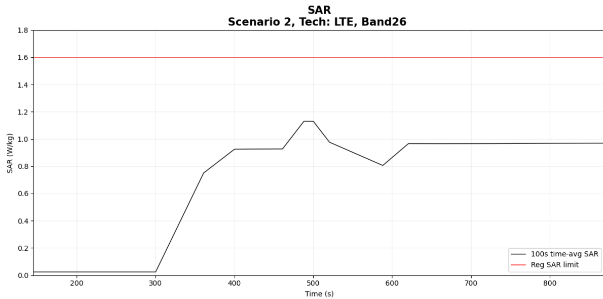
Figure 6- 24 Time-averaged SAR
