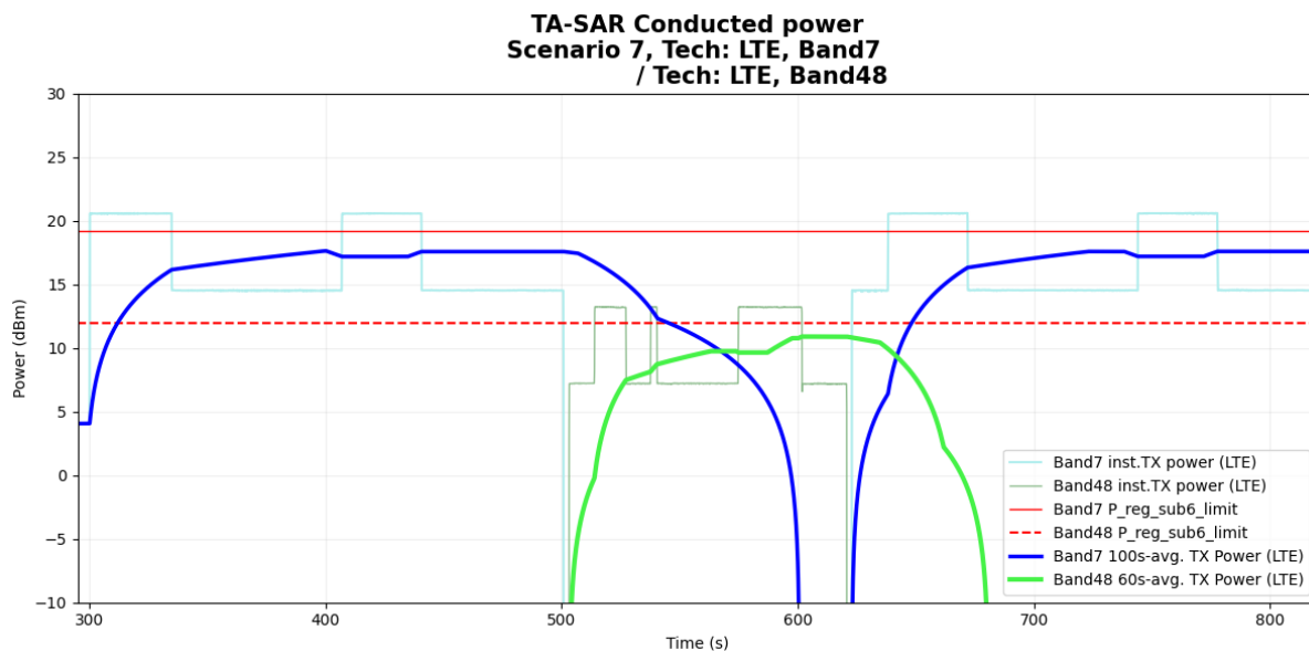
Figure 6- 47 Time-averaged conducted TX power over time
