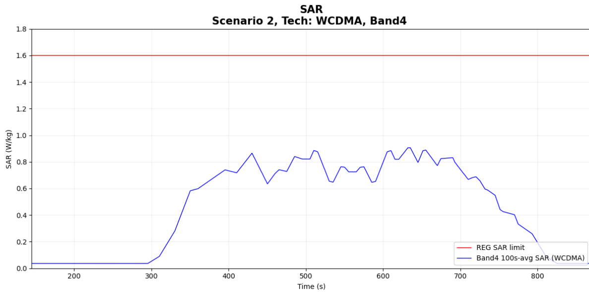
Figure 7-9 Time-averaged SAR
