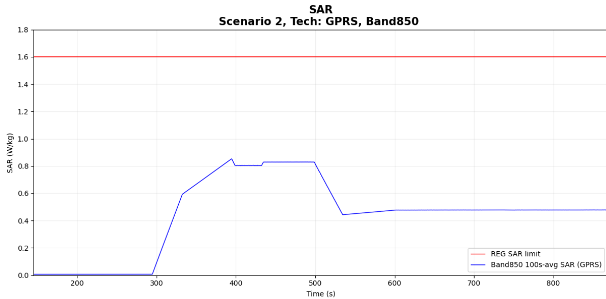
Figure 7-2 Time-averaged SAR
