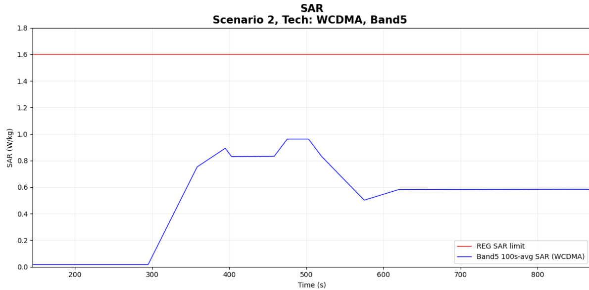
Figure 7-6 Time-averaged SAR
