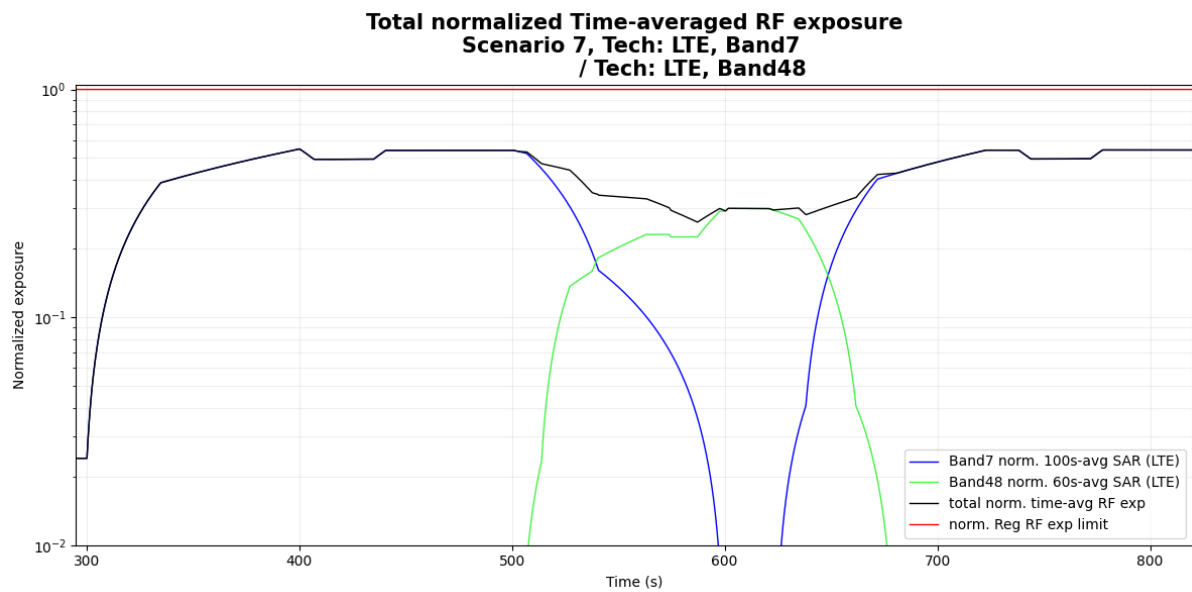
Figure 6- 48 Normalized time-averaged SAR
