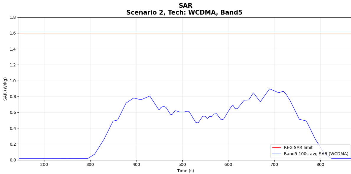
Figure 7-7 Time-averaged SAR
