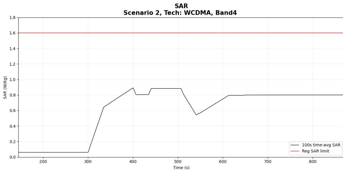
Figure 6- 20 Time-averaged SAR
