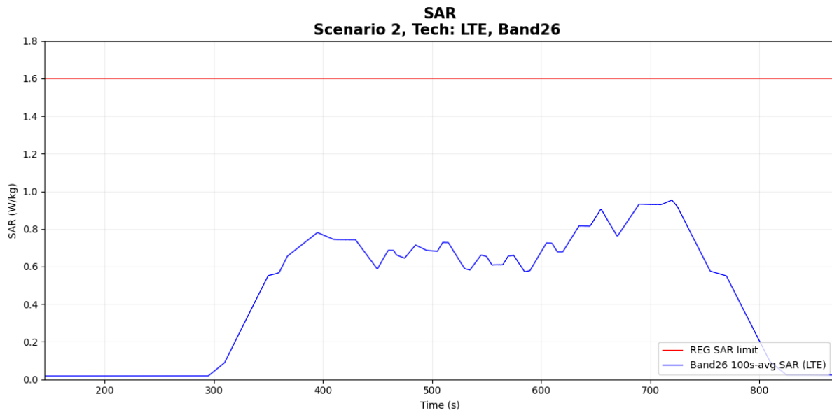
Figure 7-11 Time-averaged SAR
