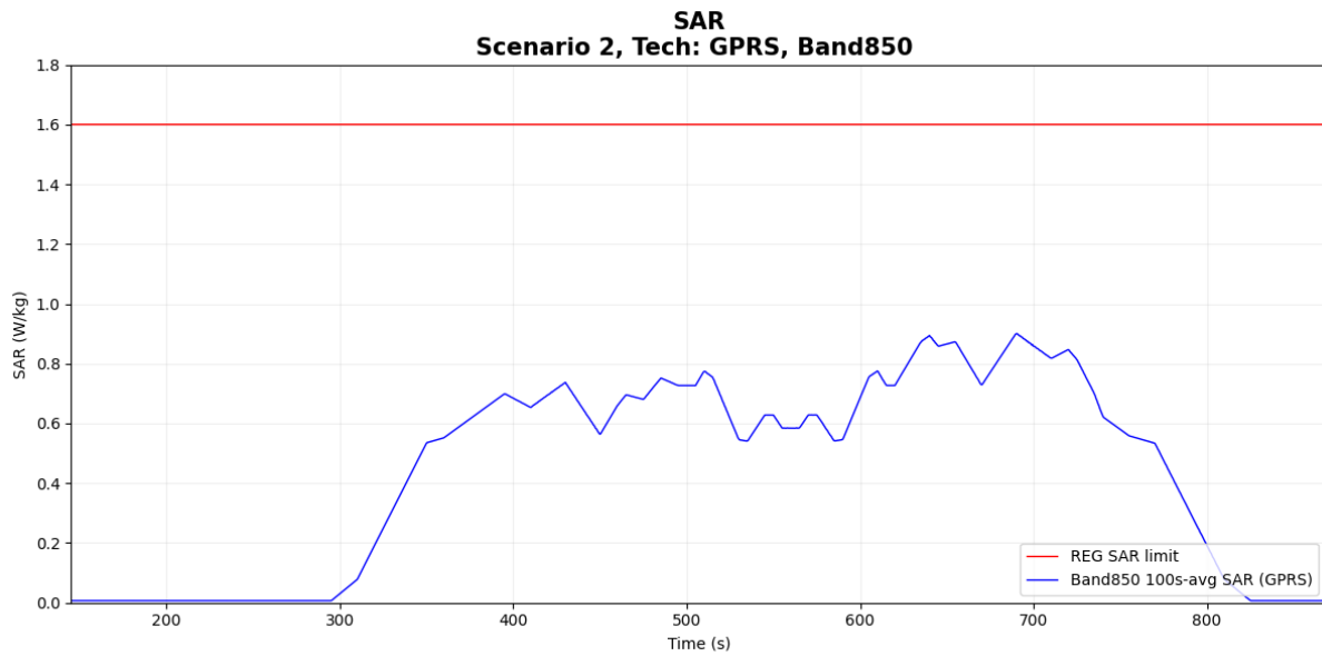
Figure 7-3 Time-averaged SAR
