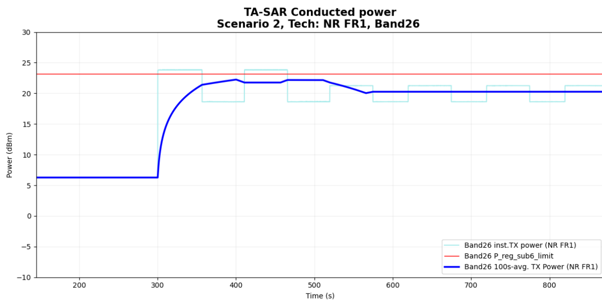
Figure 6- 31 Time-averaged conducted TX power over time
