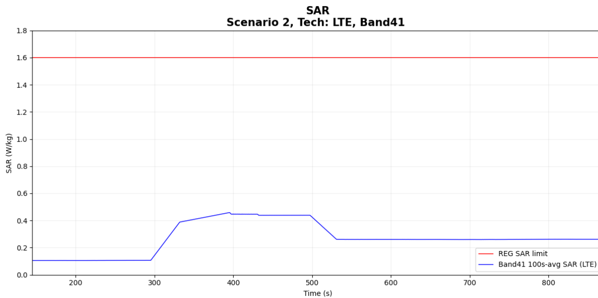
Figure 7-12 Time-averaged SAR
