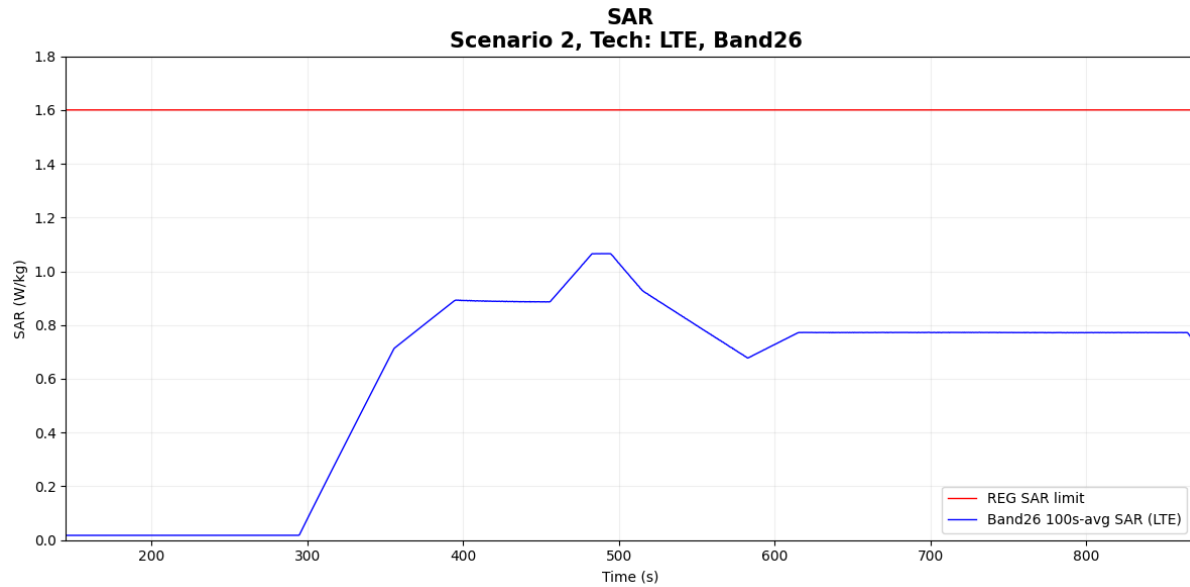
Figure 7-10 Time-averaged SAR
