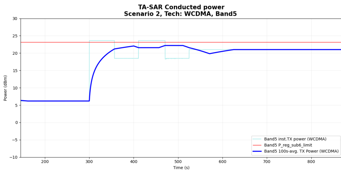
Figure 6- 15 Time-averaged conducted TX power over time
