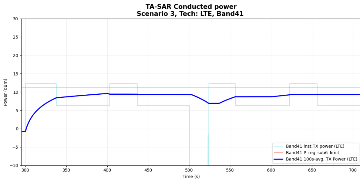
Figure 6- 39 Time-averaged conducted TX power over time
