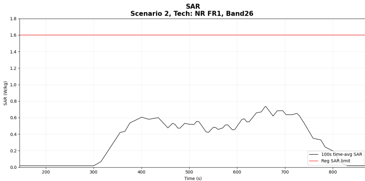
Figure 6- 34 Time-averaged SAR
