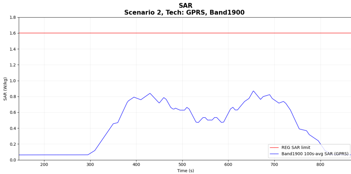
Figure 7-5 Time-averaged SAR
