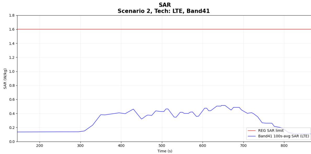
Figure 7-13 Time-averaged SAR
