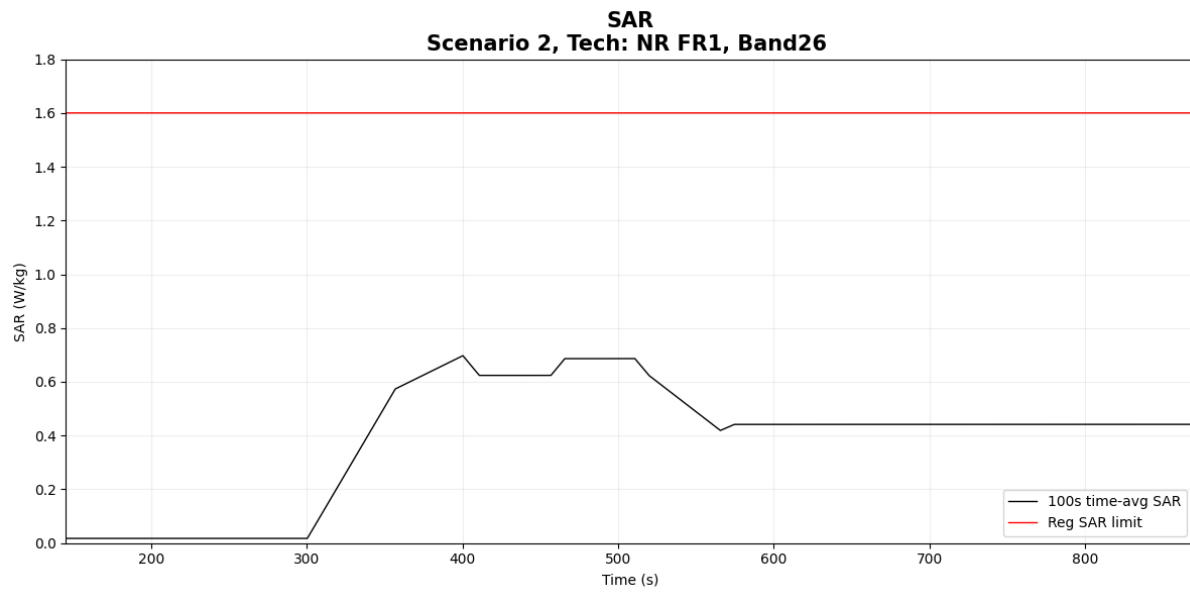
Figure 6- 32 Time-averaged SAR
