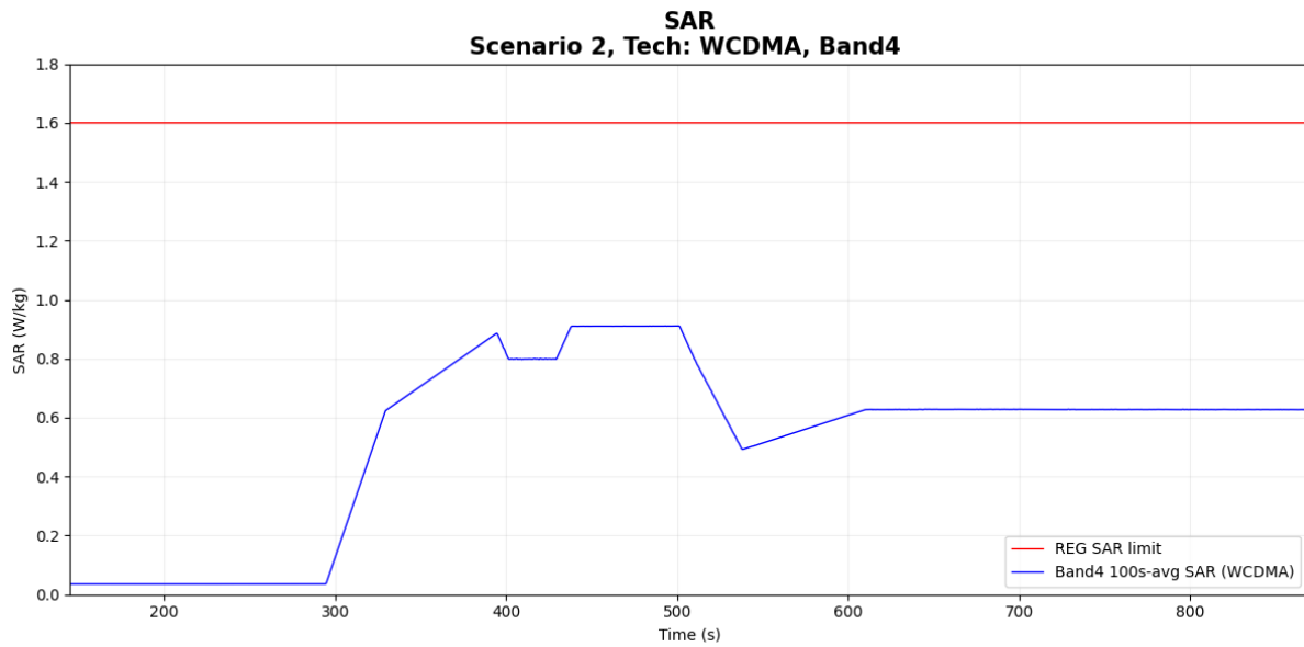
Figure 7-8 Time-averaged SAR
