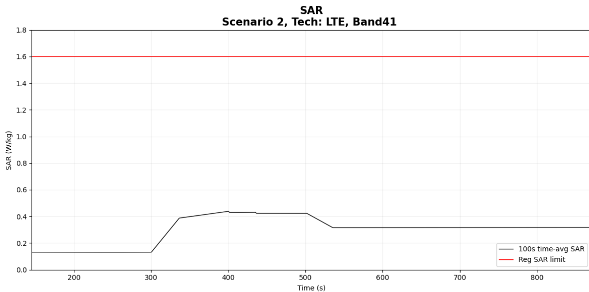
Figure 6- 28 Time-averaged SAR
