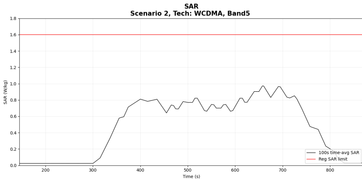
Figure 6- 18 Time-averaged SAR
