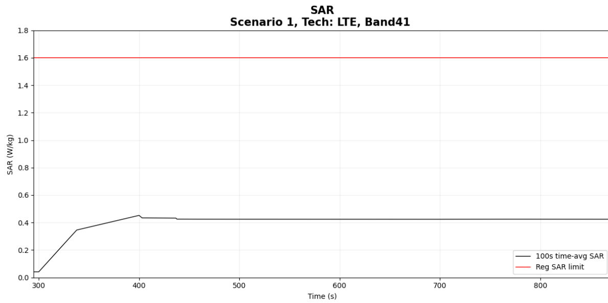
Figure 6- 6 Time-averaged SAR
