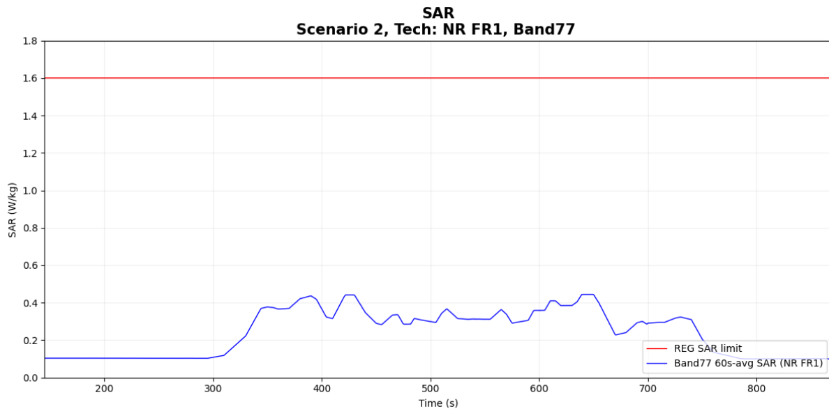
Figure 7-17 Time-averaged SAR for case
