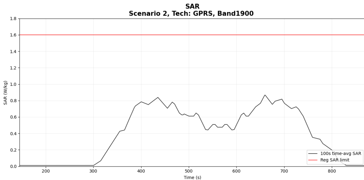
Figure 6- 14 Time-averaged SAR
