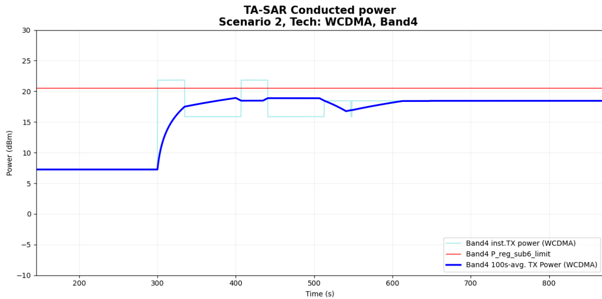
Figure 6- 19 Time-averaged conducted TX power over time
