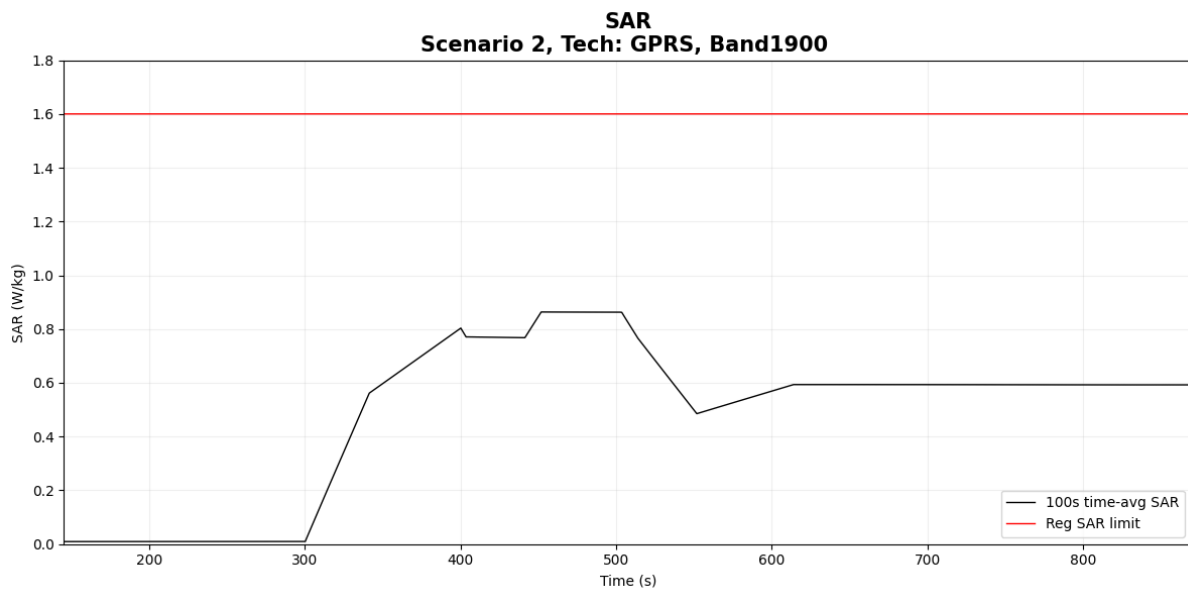
Figure 6- 12 Time-averaged SAR
