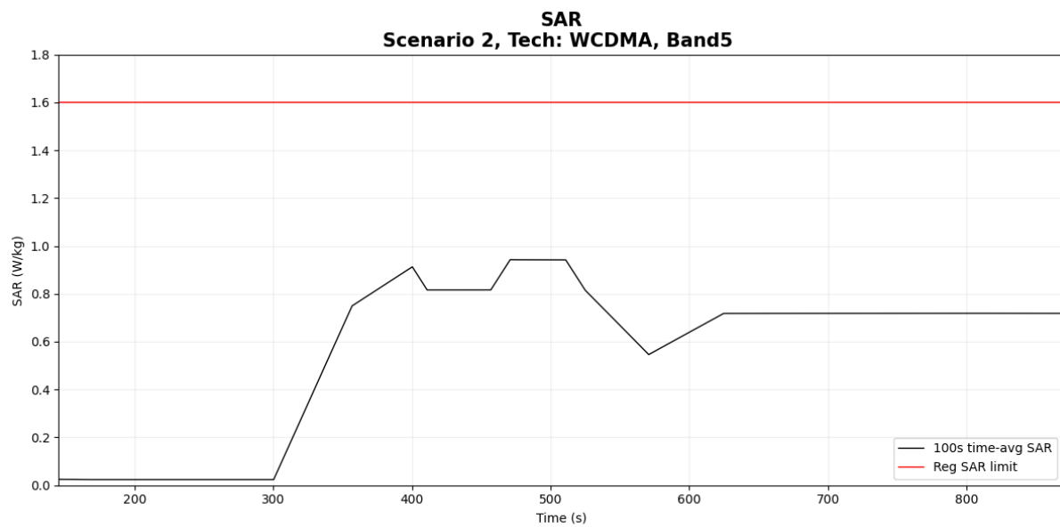
figure 6- 16 Time-averaged SAR
