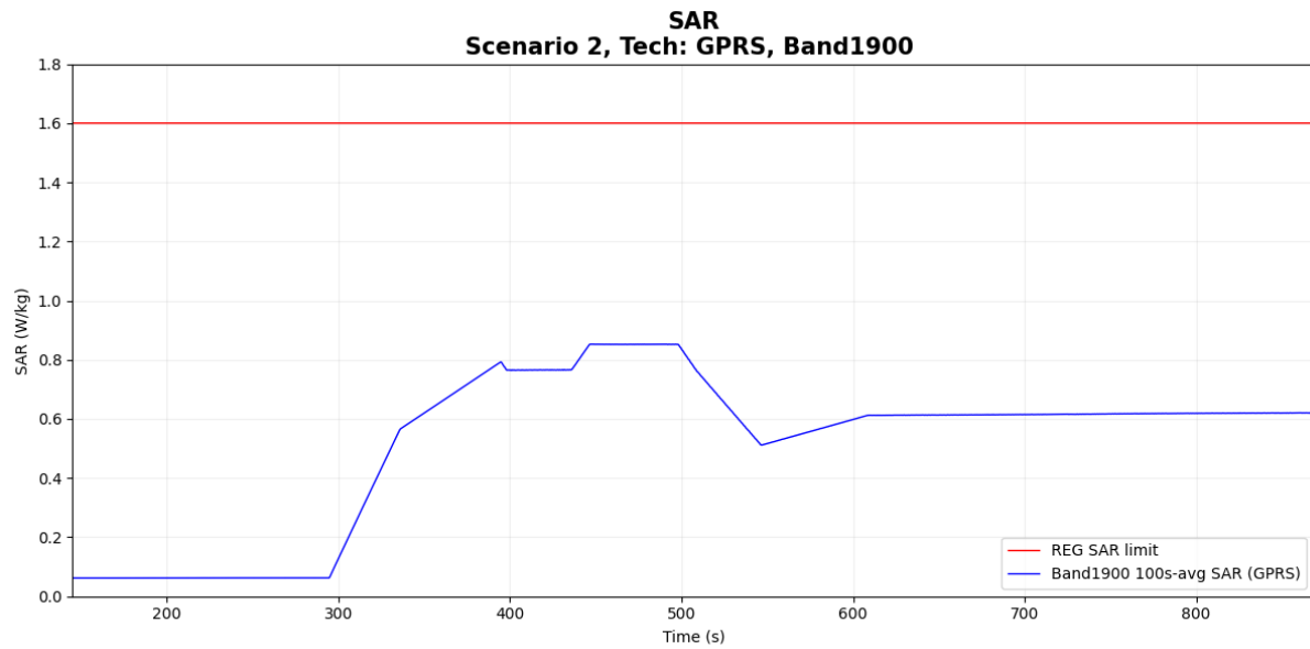
Figure 7-4 Time-averaged SAR
