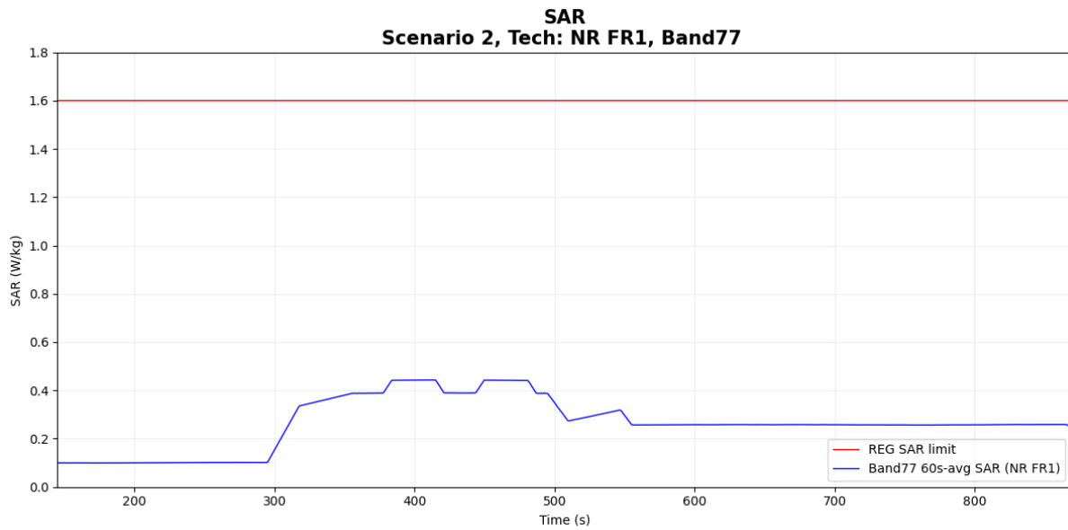
Figure 7-16 Time-averaged SAR
