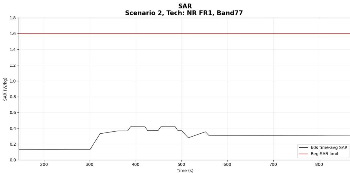
Figure 6- 36 Time-averaged SAR
