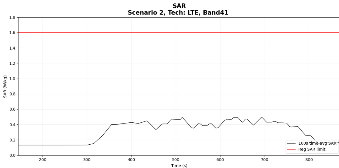
Figure 6- 30 Time-averaged SAR
