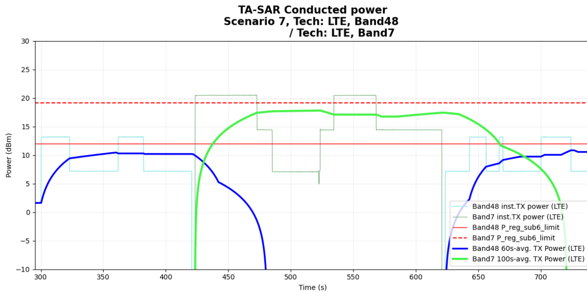
Figure 6- 45 Time-averaged conducted TX power over time
