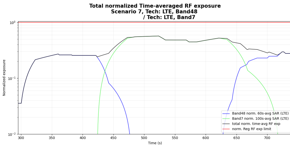
Figure 6- 46 Normalized time-averaged SAR
