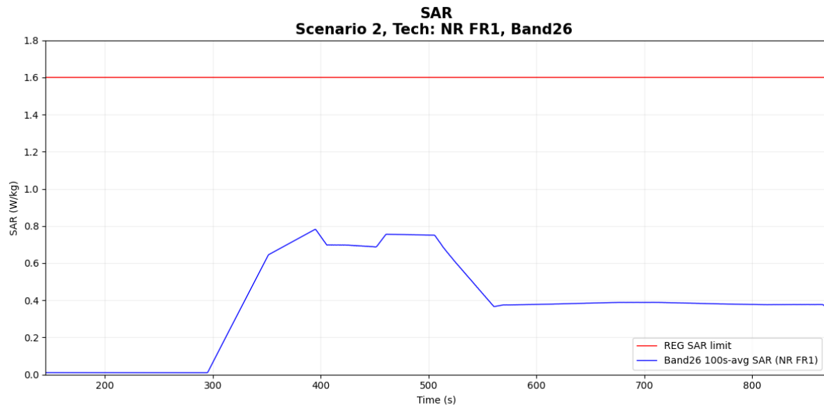
Figure 7-14 Time-averaged SAR
