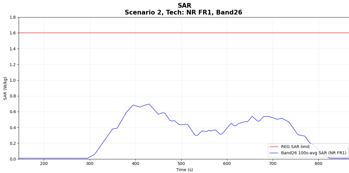
Figure 7-15 Time-averaged SAR
