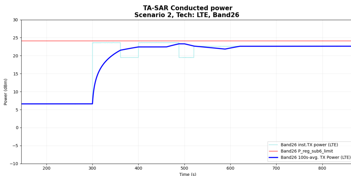
Figure 6- 23 Time-averaged conducted TX power over time
