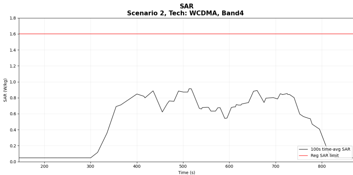
Figure 6- 22 Time-averaged SAR
