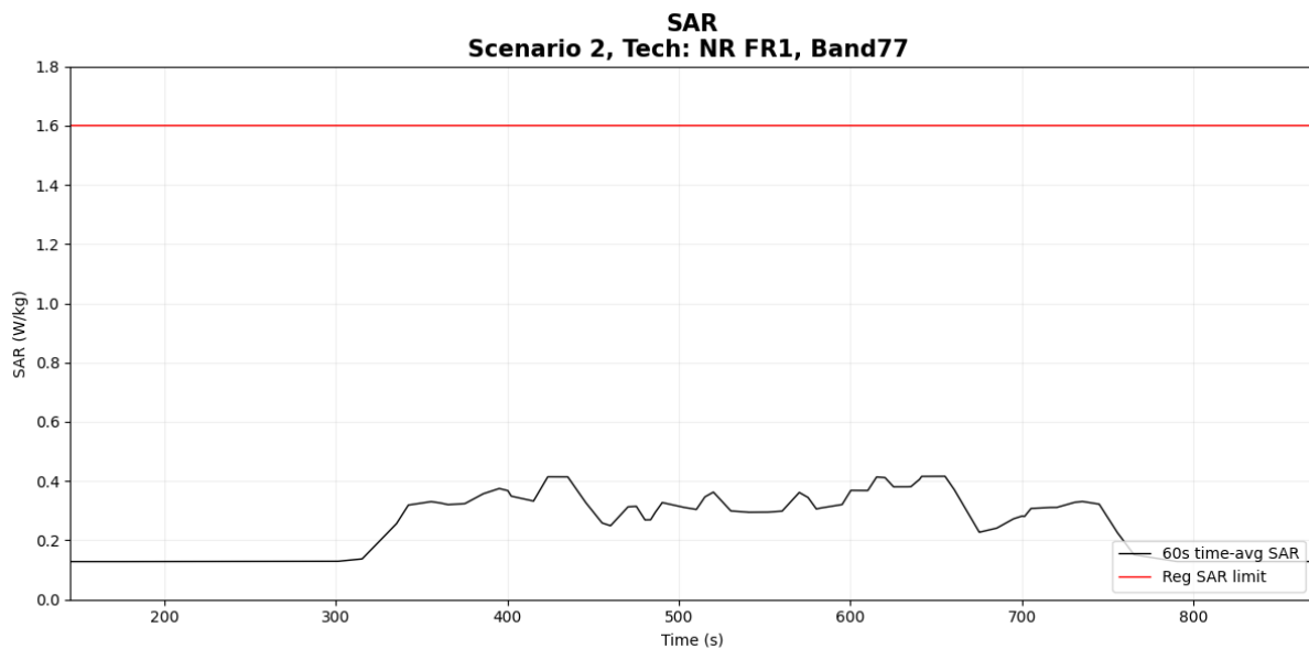
Figure 6- 38 Time-averaged SAR
