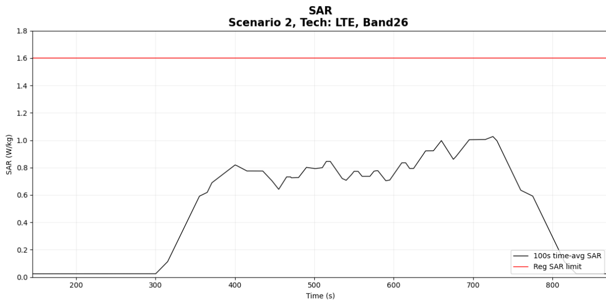
Figure 6- 26 Time-averaged SAR
