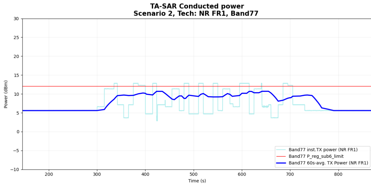
Figure 6- 37 Time-averaged conducted TX power over time
