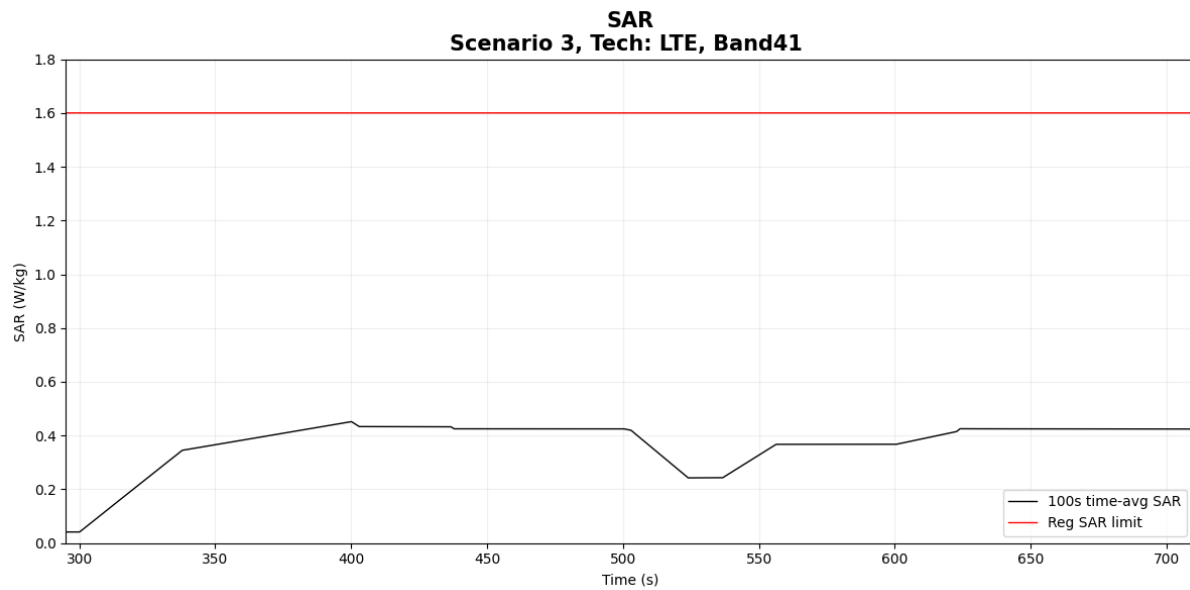
Figure 6- 40 Time-averaged SAR
