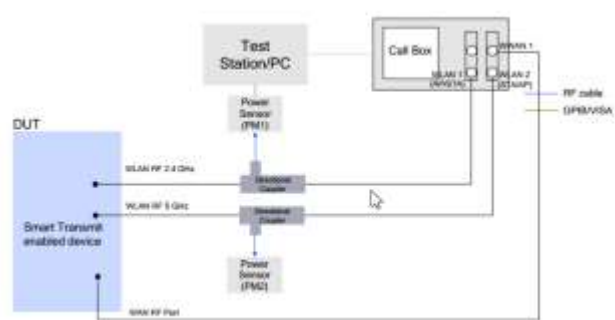
WLAN DBS Test Setup – SISO
