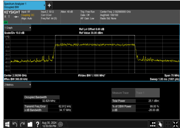
N41(35M)_CP-OFDM_256 QAM_Outer_Full_Mid_CH
