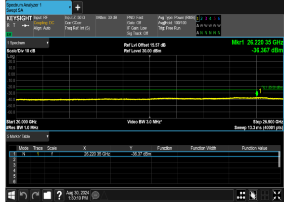
N41(100M)_DFT-s-OFDM_QPSK_Edge_1RB_Left_Mid_CH
