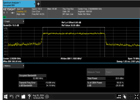
N41(35M)_CP-OFDM_16 QAM_Outer_Full_Mid_CH
