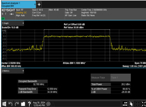
N41(35M)_CP-OFDM_64 QAM_Outer_Full_Mid_CH
