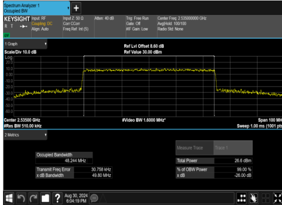
N7(50M)_CP- OFDM_QPSK_Outer_Full_Mid_CH
