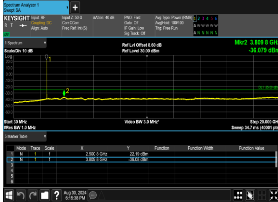
N7(25M)_DFT-s-OFDM_BPSK_Edge_1RB_Left_Low_CH
