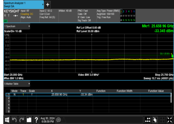
N7(5M)_DFT-s-OFDM_BPSK_Edge_1RB_Left_Low_CH
