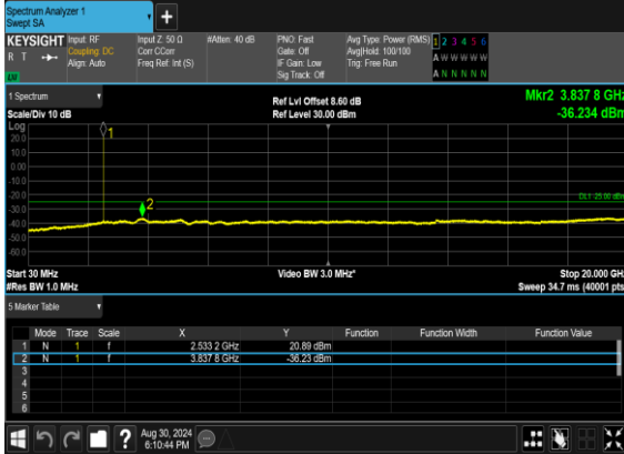
N7(5M)_DFT-s-OFDM_QPSK_Edge_1RB_Left_Mid_CH
