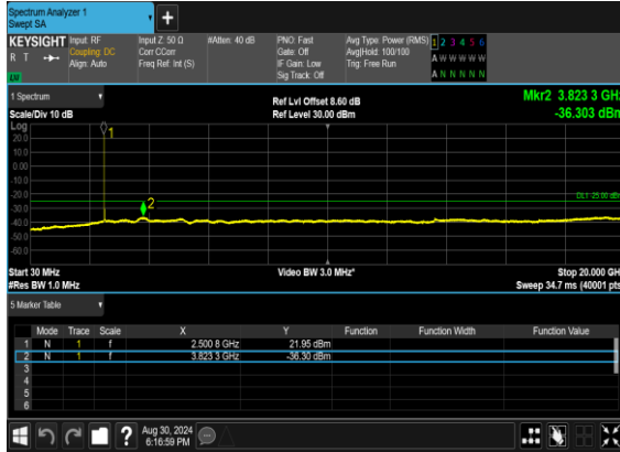
N7(25M)_DFT-s-OFDM_QPSK_Edge_1RB_Left_Low_CH
