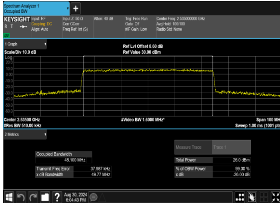
N7(50M)_CP-OFDM_64 QAM_Outer_Full_Mid_CH
