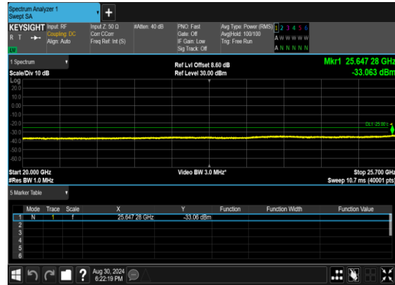
N7(25M)_DFT-s-OFDM_BPSK_Edge_1RB_Left_High_CH
