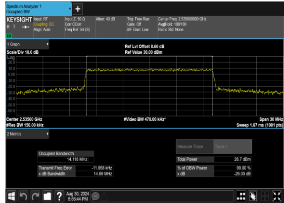
N7(15M)_CP-OFDM_16 QAM_Outer_Full_Mid_CH
