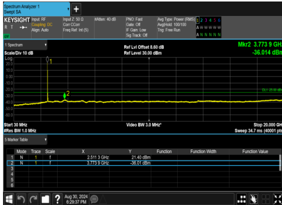
N7(50M)_DFT-s-OFDM_QPSK_Edge_1RB_Left_Mid_CH
