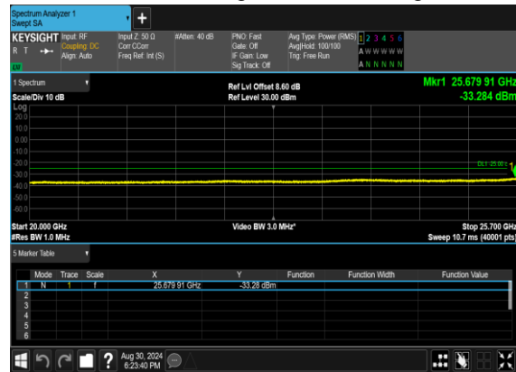
N7(25M)_DFT-s-OFDM_QPSK_Edge_1RB_Left_High_CH
