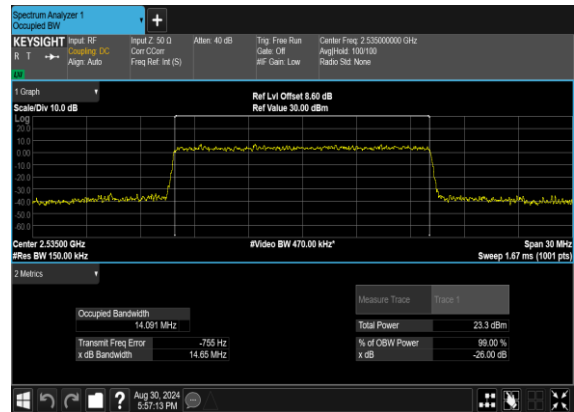
N7(15M)_CP-OFDM_256 QAM_Outer_Full_Mid_CH
