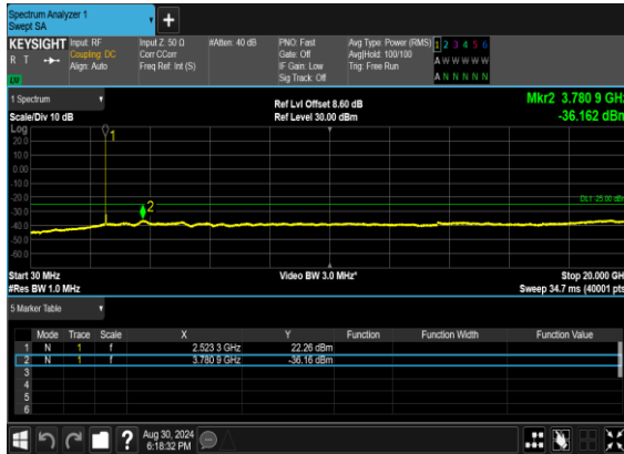
N7(25M)_DFT-s-OFDM_BPSK_Edge_1RB_Left_Mid_CH
