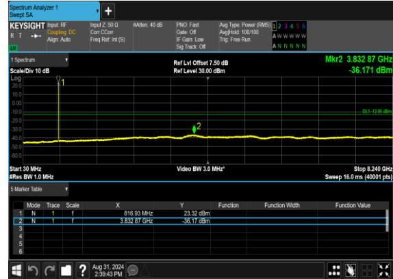
N26(5M)_DFT-s-OFDM_QPSK_Edge_1RB_Left_Mid_CH
