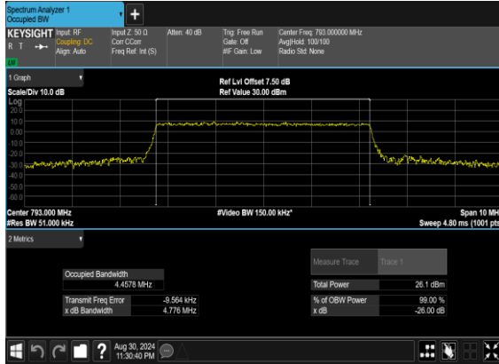
N14(5M)_CP-OFDM_QPSK_Outer_Full_Mid_CH
