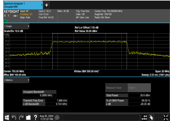
N14(10M)_CP-OFDM_16 QAM_Outer_Full_Mid_CH
