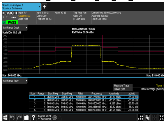
N14(10M)_DFT-s-OFDM_BPSK_Outer_Full_Mid_CH
