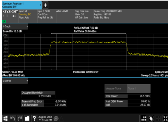
N14(10M)_CP-OFDM_QPSK_Outer_Full_Mid_CH
