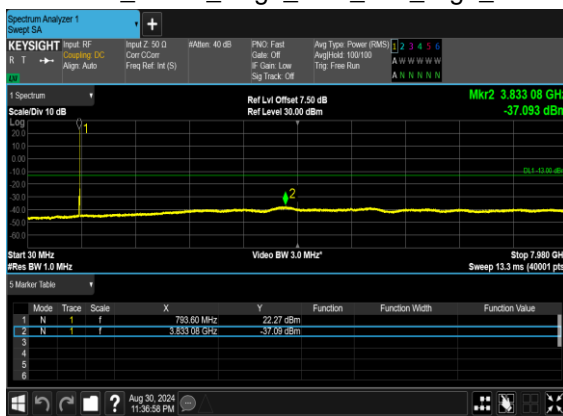
N14(5M)_DFT-s-OFDM_BPSK_Edge_1RB_Left_High_CH
