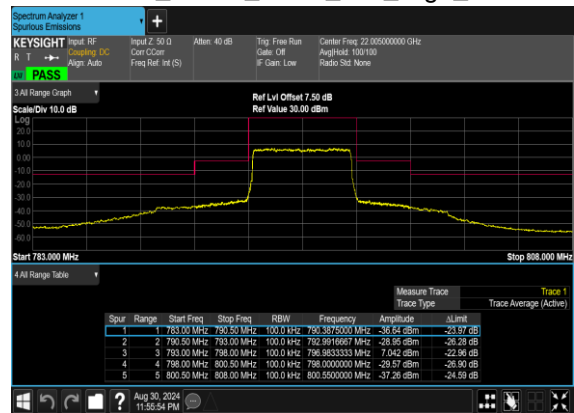
N14(5M)_DFT-s-OFDM_QPSK_Outer_Full_High_CH
