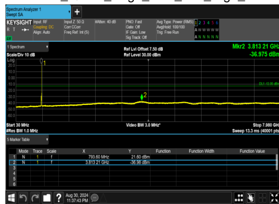
N14(5M)_DFT-s-OFDM_QPSK_Edge_1RB_Left_High_CH
