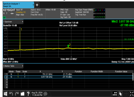
N14(5M)_DFT-s-OFDM_QPSK_Edge_1RB_Left_Mid_CH
