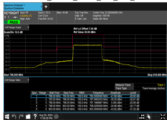
N14(10M)_DFT-s-OFDM_QPSK_Outer_Full_Mid_CH
