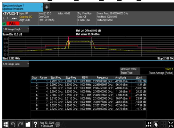
N30(5M)_DFT-s-OFDM_BPSK_Outer_Full_Low_CH
