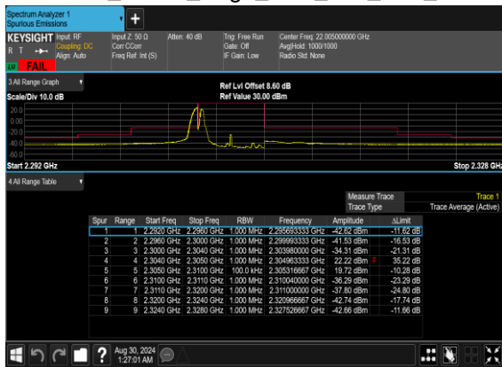
N30(5M)_DFT-s-OFDM_QPSK_Edge_1RB_Left_Low_CH
