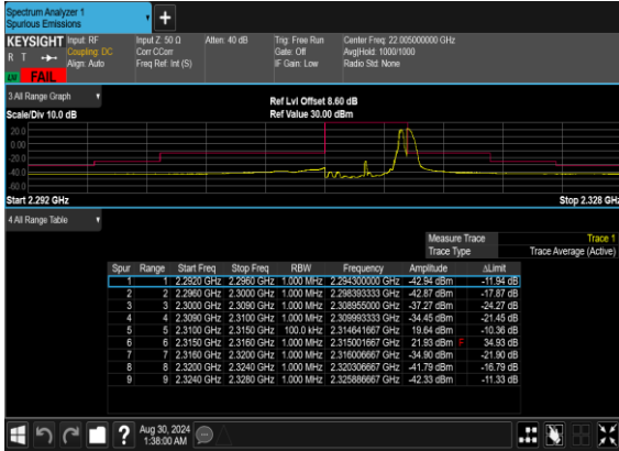
N30(5M)_DFT-s-OFDM_QPSK_Edge_1RB_Right_High_CH
