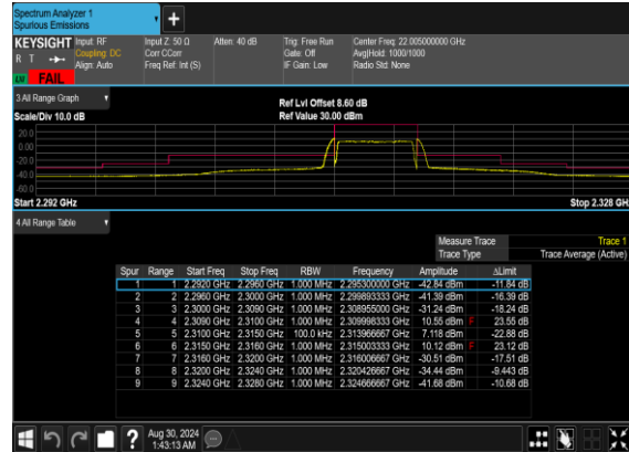
N30(5M)_DFT-s-OFDM_QPSK_Outer_Full_High_CH
