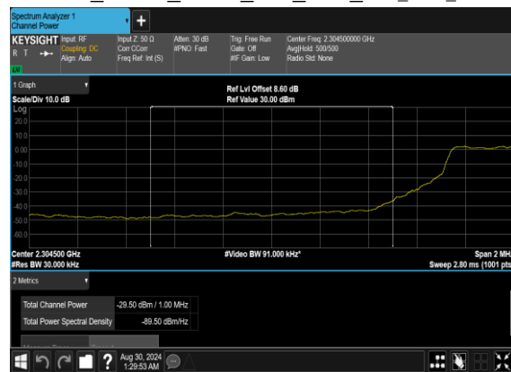
N30(5M)_DFT-s-OFDM_BPSK_Outer_Full_Low_CH_CHP_PASS
