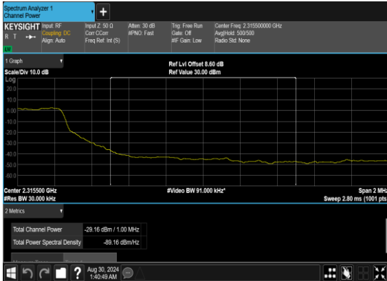
N30(5M)_DFT-s-OFDM_BPSK_Outer_Full_High_CH_CHP_PASS
