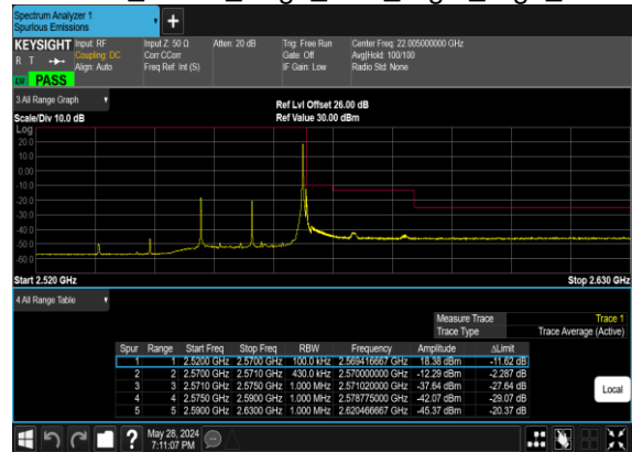
B2_N7(20M)_DFT-s-OFDM_QPSK_Edge_1RB_Right_High_CH
