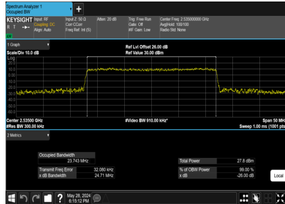
B2_N7(25M)_CP-OFDM_16QAM_Outer_Full_Mid_CH
