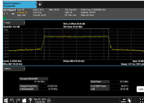
B2_N7(15M)_CP-OFDM_256 QAM_Outer_Full_Mid_CH
