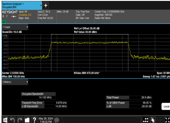
B2_N7(15M)_CP-OFDM_64 QAM_Outer_Full_Mid_CH
