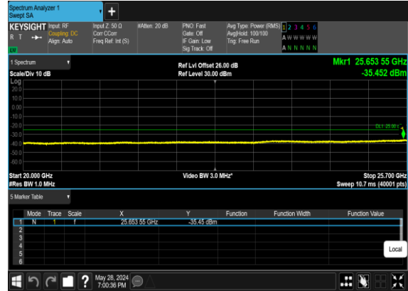
B2_N7(50M)_DFT-s-OFDM_BPSK_Edge_1RB_Left_High_CH
