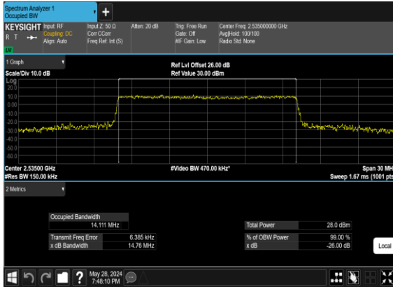
B2_N7(15M)_CP-OFDM_QPSK_Outer_Full_Mid_CH
