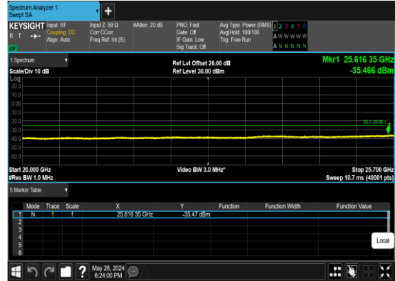
B2_N7(5M)_DFT-s-OFDM_QPSK_Edge_1RB_Left_Mid_CH
