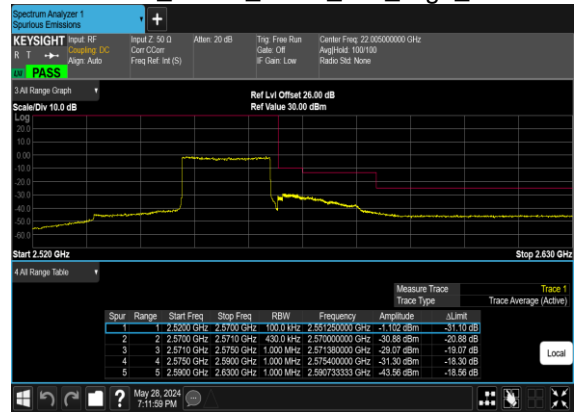
B2_N7(20M)_DFT-s-OFDM_QPSK_Outer_Full_High_CH
