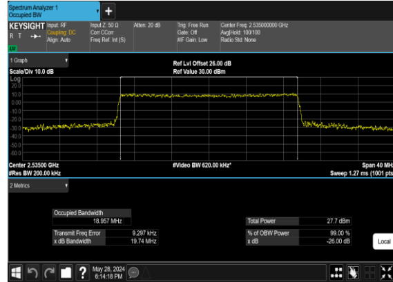
B2_N7(20M)_CP-OFDM_16QAM_Outer_Full_Mid_CH
