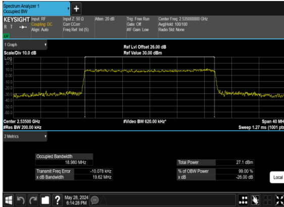
B2_N7(20M)_CP-OFDM_64QAM_Outer_Full_Mid_CH
