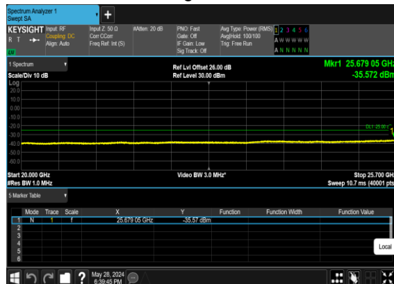
B2_N7(50M)_DFT-s-OFDM_BPSK_Edge_1RB_Left_Mid_CH
