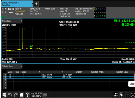
B2_N7(20M)_DFT-s-OFDM_BPSK_Edge_1RB_Left_Low_CH
