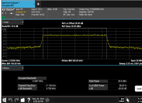
B2_N7(10M)_CP-OFDM_64 QAM_Outer_Full_Mid_CH
