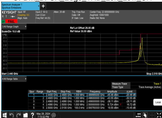
B2_N7(50M)_DFT-s-OFDM_BPSK_Edge_1RB_Left_Low_CH
