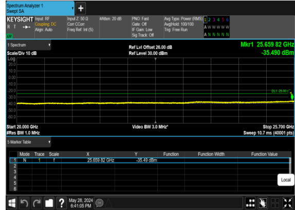
B2_N7(50M)_DFT-s-OFDM_QPSK_Edge_1RB_Left_Mid_CH
