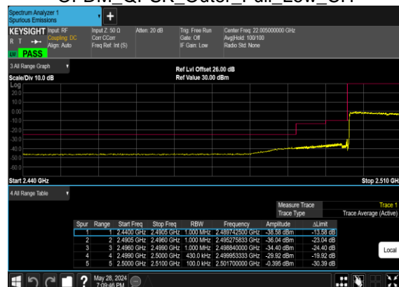
B2_N7(20M)_DFT-s-OFDM_QPSK_Outer_Full_Low_CH
