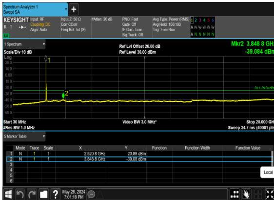
B2_N7(50M)_DFT-s-OFDM_QPSK_Edge_1RB_Left_High_CH
