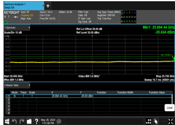
B2_N7(50M)_DFT-s-OFDM_QPSK_Edge_1RB_Left_High_CH
