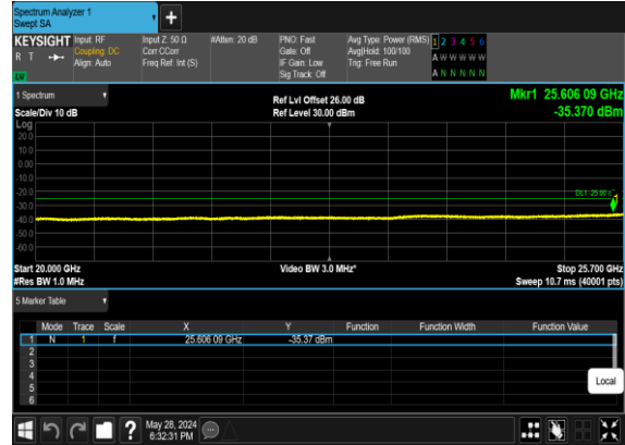
B2_N7(20M)_DFT-s-OFDM_QPSK_Edge_1RB_Left_Mid_CH
