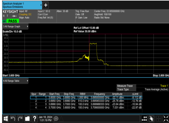
N77(10M)_DFT-s- OFDM_BPSK_Outer_Full_Low_CH
