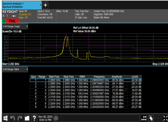
N30(5M)_DFT-s-OFDM_QPSK_Edge_1RB_Left_Low_CH
