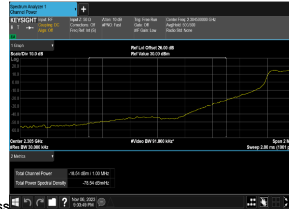
N30(10M)_DFT-s-OFDM_QPSK_Edge_1RB_Left_Low_CH_CHP_PA
