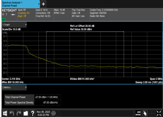
N30(5M)_DFT-s-OFDM_QPSK_Outer_Full_High_CH_CHP_PASS
