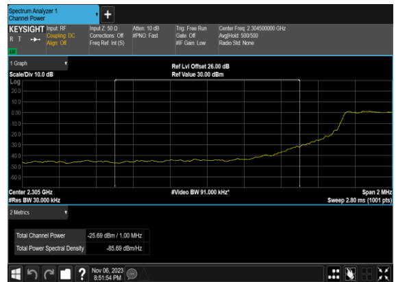
N30(5M)_DFT-s-OFDM_BPSK_Outer_Full_Low_CH_CHP_PASS
