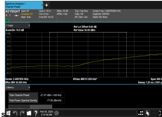
N7(20M)_DFT-s- OFDM_QPSK_Edge_1RB_Left_Low_CH_CHP_PAS
