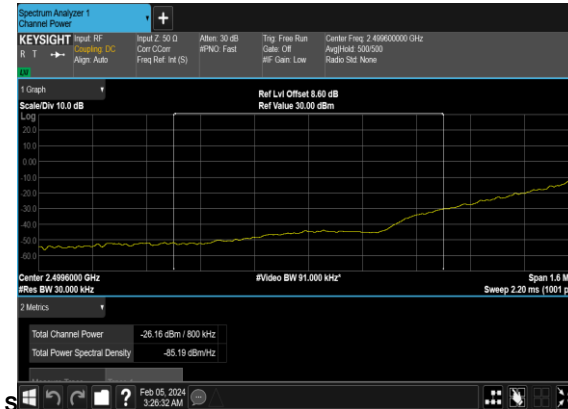
N7(40M)_DFT-s-OFDM_QPSK_Edge_1RB_Left_Low_CH_CHP_PAS
