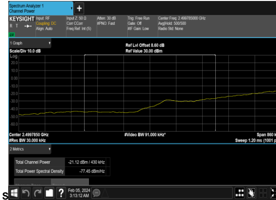
N7(20M)_DFT-s- OFDM_BPSK_Edge_1RB_Left_Low_CH_CHP_PAS
