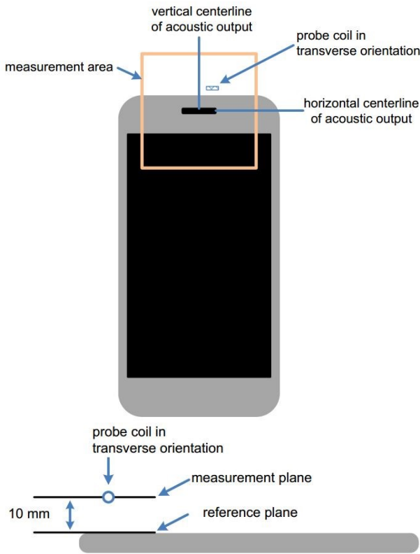
Measurement and reference planes probe orientation for WD audio frequency magnetic field measurements
