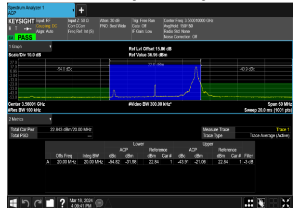
N48(20M)_DFT-s-OFDM_QPSK_Edge_1RB_Right_Low_CH
