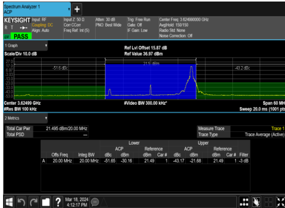
N48(20M)_DFT-s-OFDM_PI_2-BPSK_Edge_1RB_Right_Mid_CH
