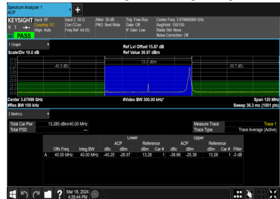
N48(40M)_DFT-s-OFDM_QPSK_Edge_1RB_Right_High_CH
