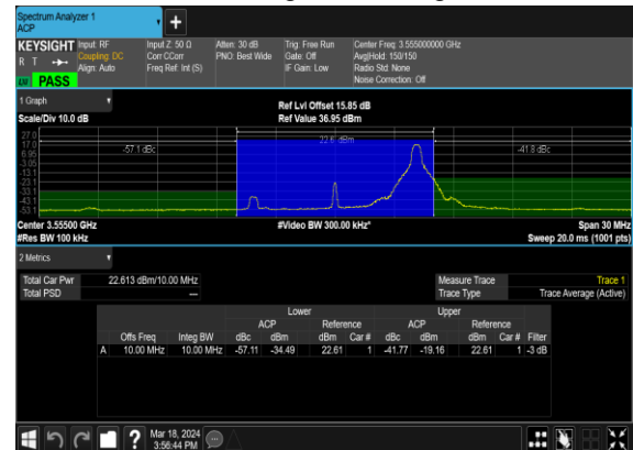
N48(10M)_DFT-s-OFDM_QPSK_Edge_1RB_Right_Low_CH
