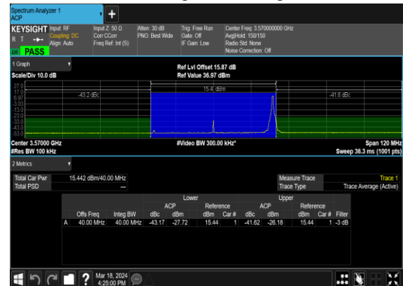
N48(40M)_DFT-s-OFDM_QPSK_Edge_1RB_Right_Low_CH
