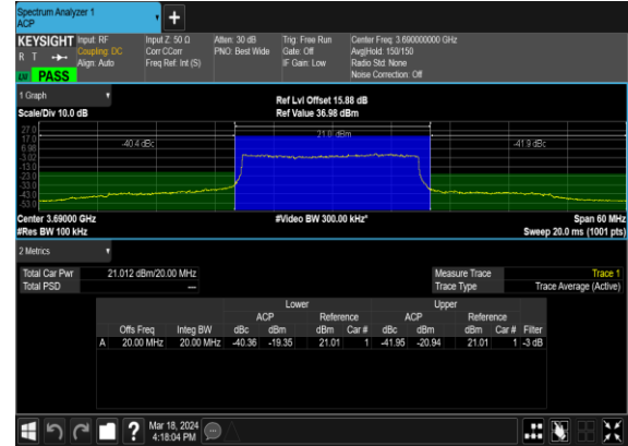
N48(20M)_DFT-s-OFDM_QPSK_Outer_Full_High_CH
