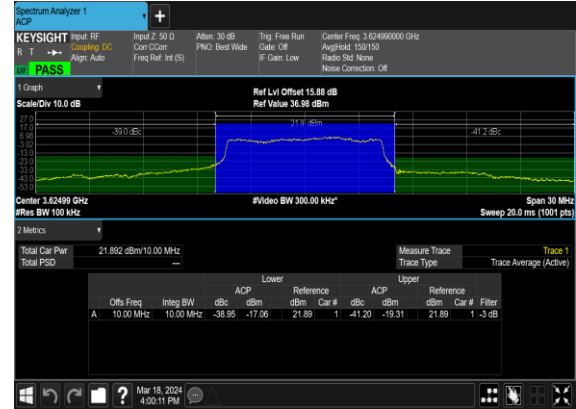
N48(10M)_DFT-s-OFDM_QPSK_Outer_Full_Mid_CH
