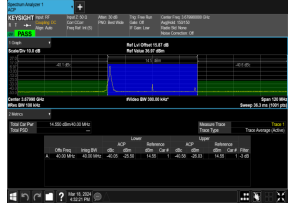
N48(40M)_DFT-s-OFDM_PI_2-BPSK_Edge_1RB_Left_High_CH
