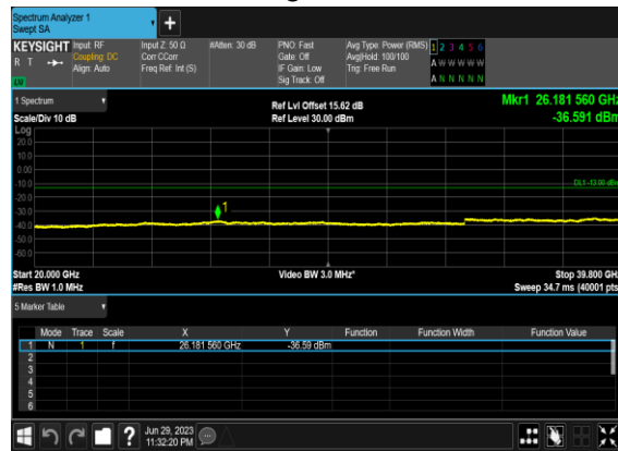
N77(20M)_DFT-s-OFDM_BPSK_Edge_1RB_Left_Mid_CH
