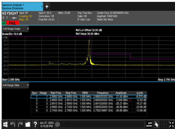
N41(50M)_DFT-s- OFDM_BPSK_Edge_1RB_Right_High_CH
