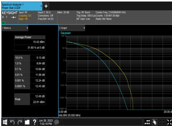
N41(100M)_DFT-s-OFDM_QPSK_Outer_Full_Mid_CH
