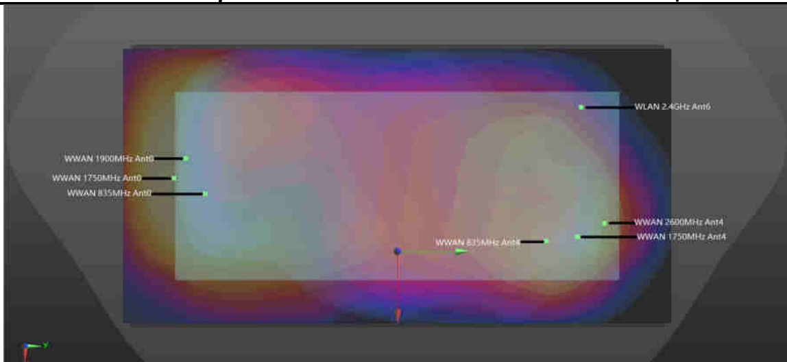
WWAN Ant0+WWAN Ant4+2.4GHz WIFI Back 5mm
