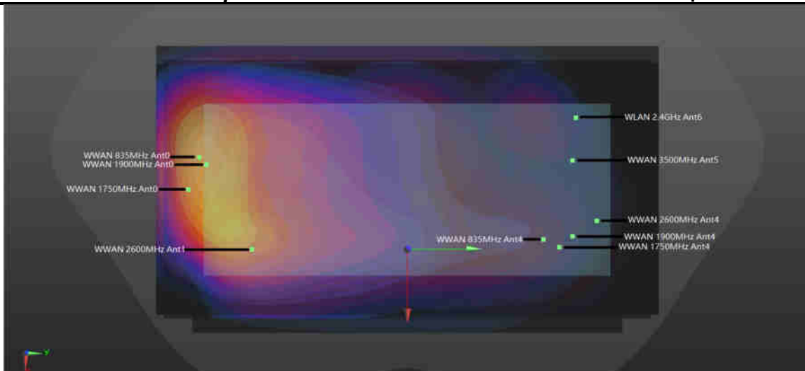
WWAN+FR1+2.4GHz WIFI Back 5mm
