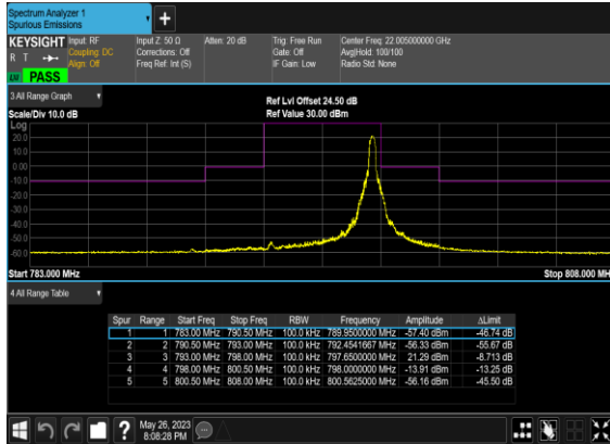
N14(5M)_DFT-s- OFDM_BPSK_Edge_1RB_Right_High_CH
