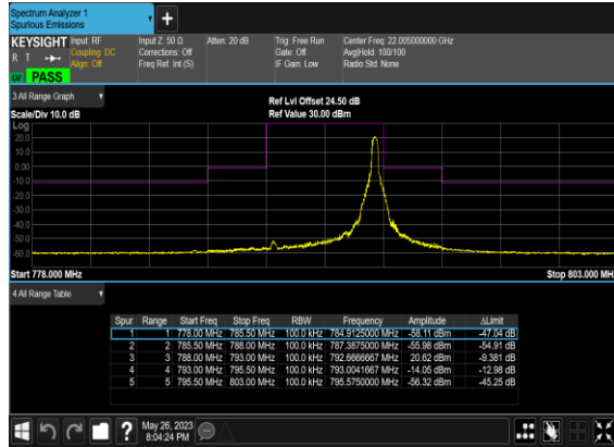
N14(5M)_DFT-s-OFDM_QPSK_Edge_1RB_Right_Low_CH
