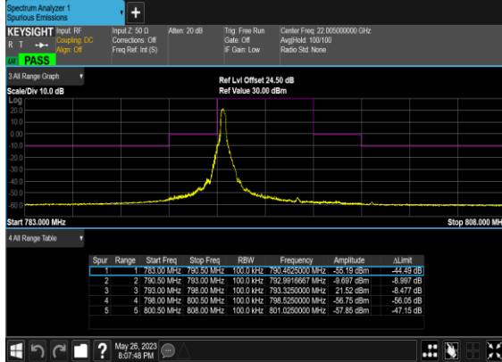
N14(5M)_DFT-s- OFDM_BPSK_Edge_1RB_Left_High_CH
