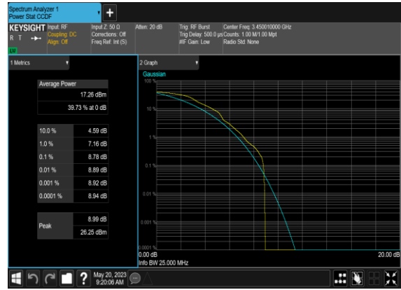
N77(100M)_DFT-s-OFDM_QPSK_Edge_1RB_Left_Mid_CH
