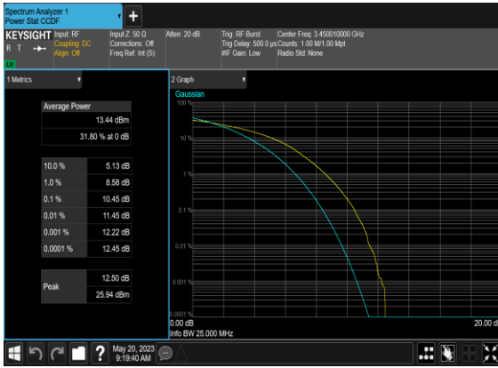
N77(100M)_DFT-s-OFDM_QPSK_Outer_Full_Mid_CH
