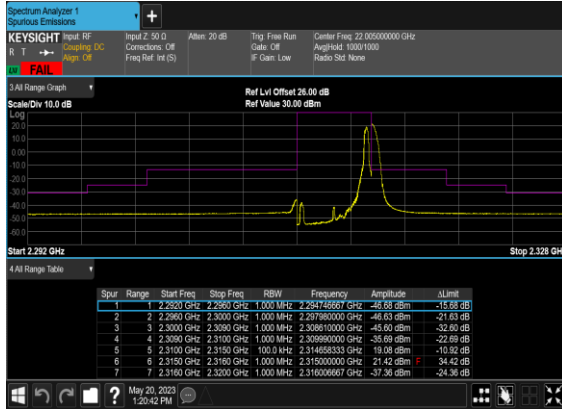
N30(5M)_DFT-s-OFDM_BPSK_Edge_1RB_Right_High_CH
