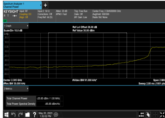
N30(10M)_DFT-s- OFDM_BPSK_Outer_Full_Mid_CH_CHP_PASS
