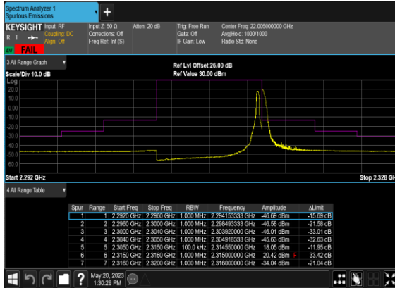
N30(10M)_DFT-s- OFDM_QPSK_Edge_1RB_Right_Mid_CH
