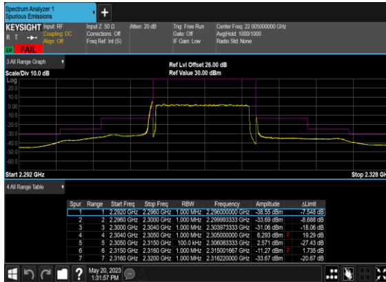
N30(10M)_DFT-s- OFDM_BPSK_Outer_Full_Mid_CH
