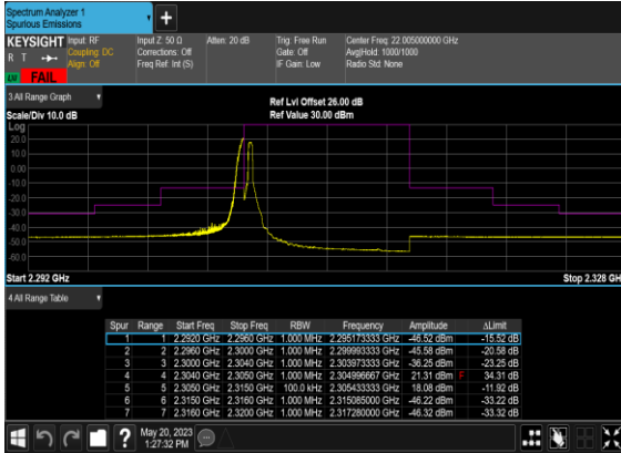
N30(10M)_DFT-s- OFDM_QPSK_Edge_1RB_Left_Mid_CH
