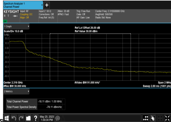
N30(10M)_DFT-s- OFDM_QPSK_Edge_1RB_Right_Mid_CH_CHP_PA
