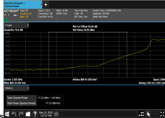
N30(10M)_DFT-s- OFDM_QPSK_Edge_1RB_Left_Mid_CH_CHP_PASS
