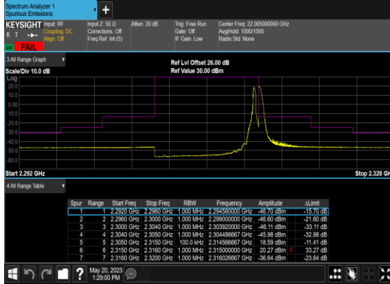
N30(10M)_DFT-s- OFDM_BPSK_Edge_1RB_Right_Mid_CH
