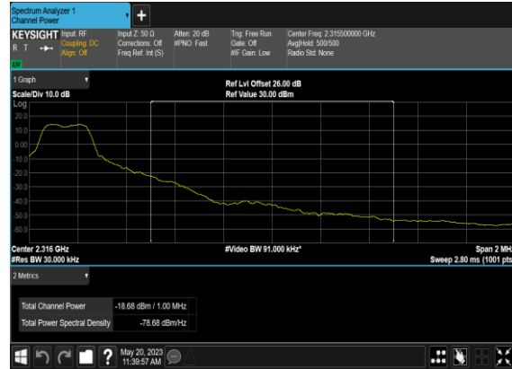
N30(5M)_DFT-s- OFDM_QPSK_Edge_1RB_Right_High_CH_CHP_P ASS
