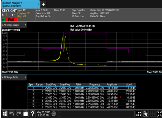
N30(10M)_DFT-s- OFDM_BPSK_Edge_1RB_Left_Mid_CH
