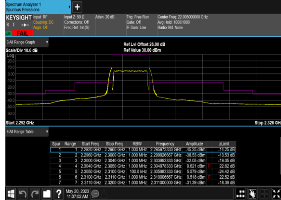
N30(5M)_DFT-s-OFDM_QPSK_Outer_Full_Low_CH
