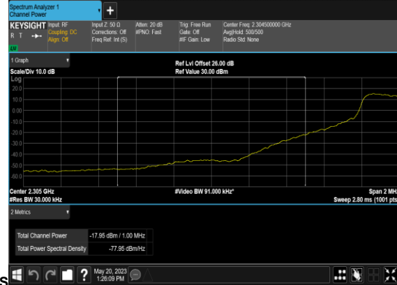
N30(10M)_DFT-s- OFDM_BPSK_Edge_1RB_Left_Mid_CH_CHP_PASS
