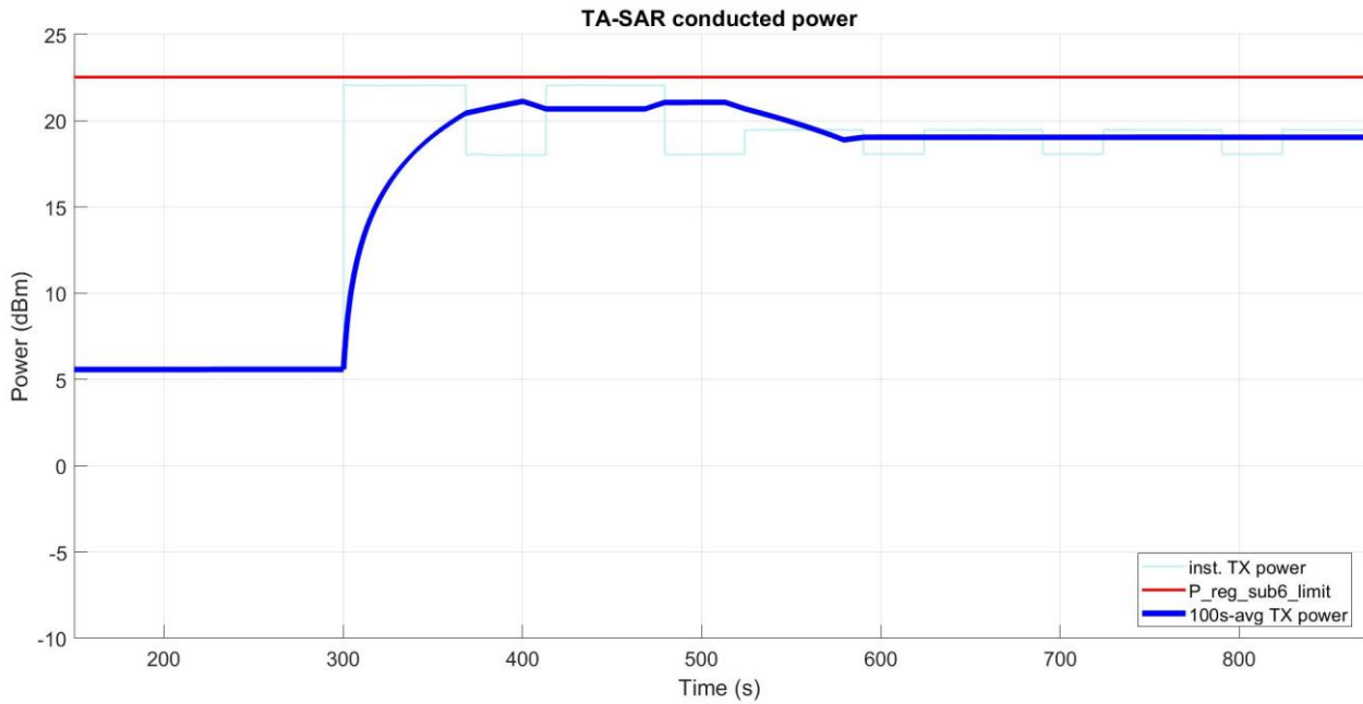
Figure 5- 33 Time-averaged conducted TX power over time
