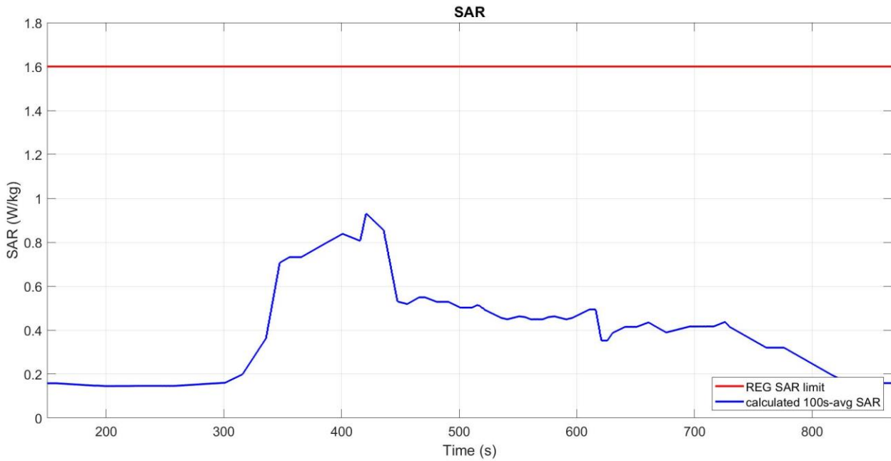
Figure 6-12 Time-averaged SAR
