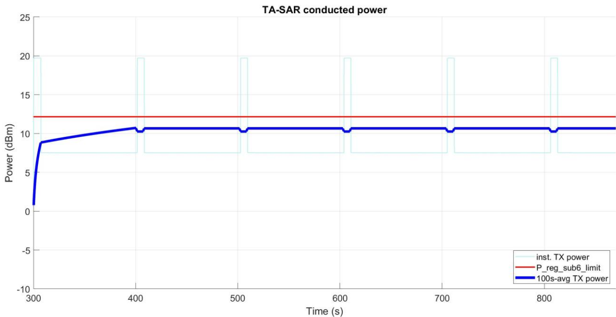
Figure 5- 5 Time-averaged conducted TX power over time
