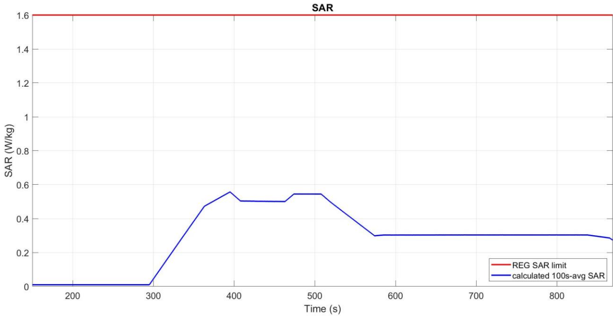
Figure 6-3 Time-averaged SAR
