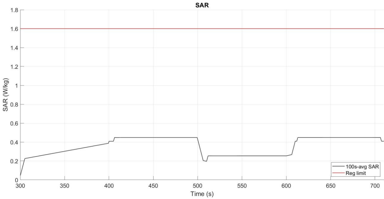
Figure 5- 37 Time-averaged SAR
