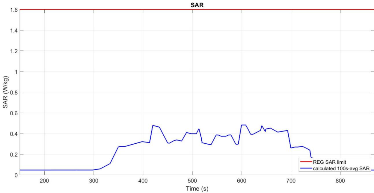
Figure 6-6 Time-averaged SAR for case
