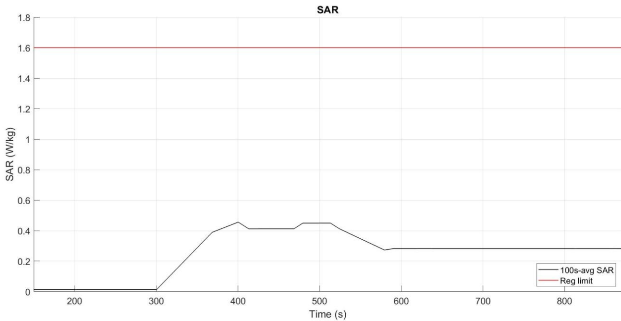
Figure 5- 34 Time-averaged SAR
