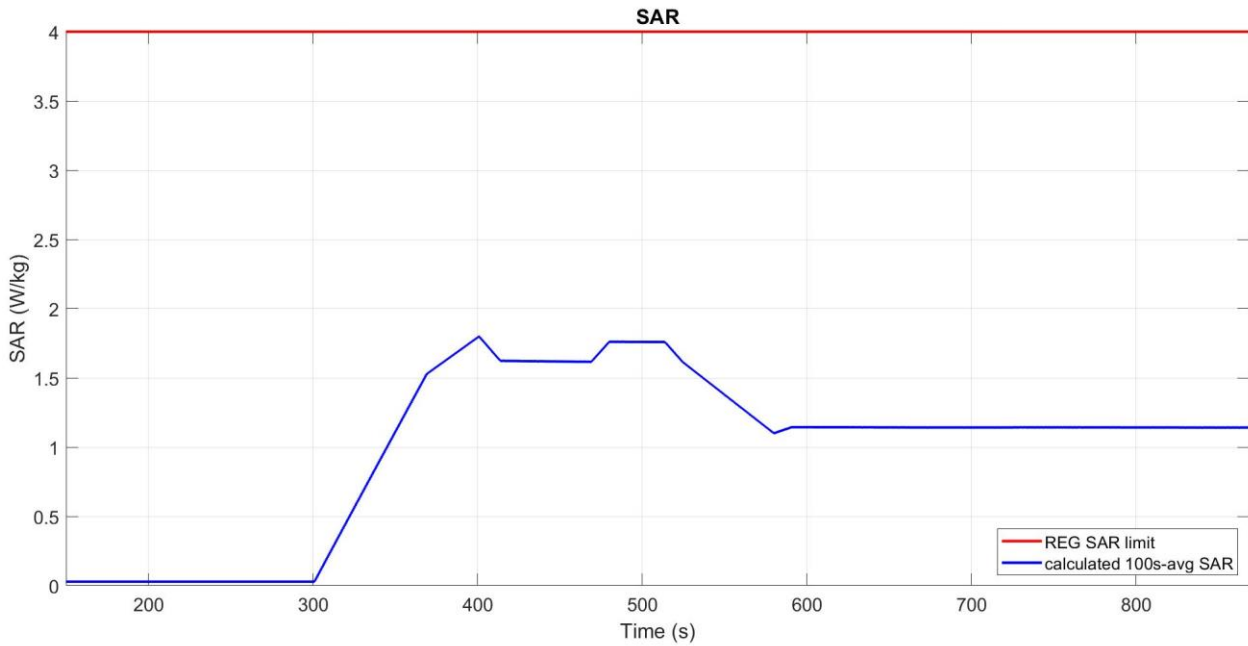
Figure 6-9 Time-averaged SAR
