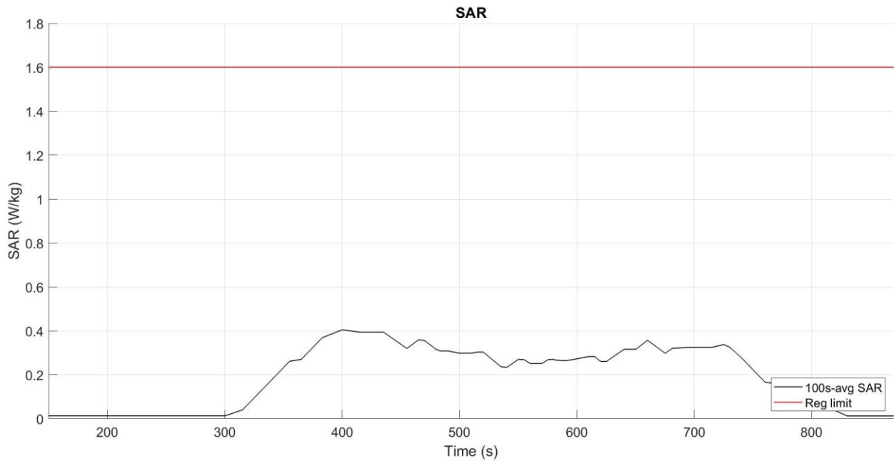
Figure 5- 36 Time-averaged SAR
