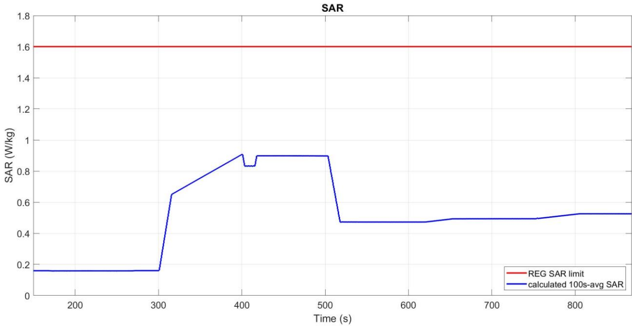
Figure 6-11 Time-averaged SAR
