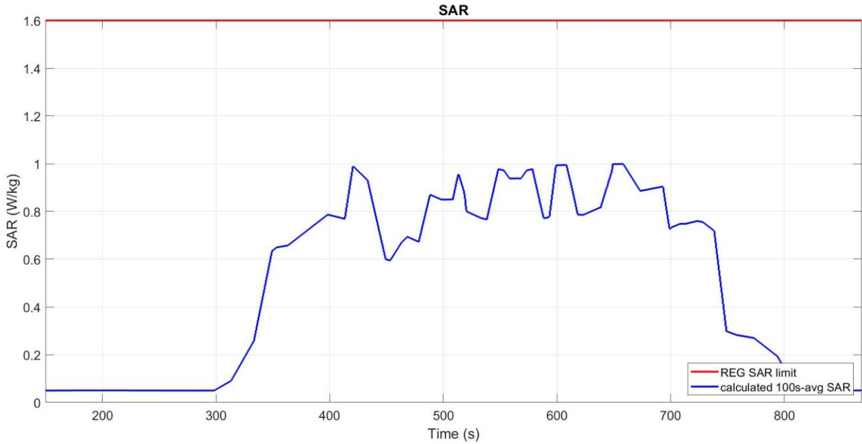
Figure 6-18 Time-averaged SAR
