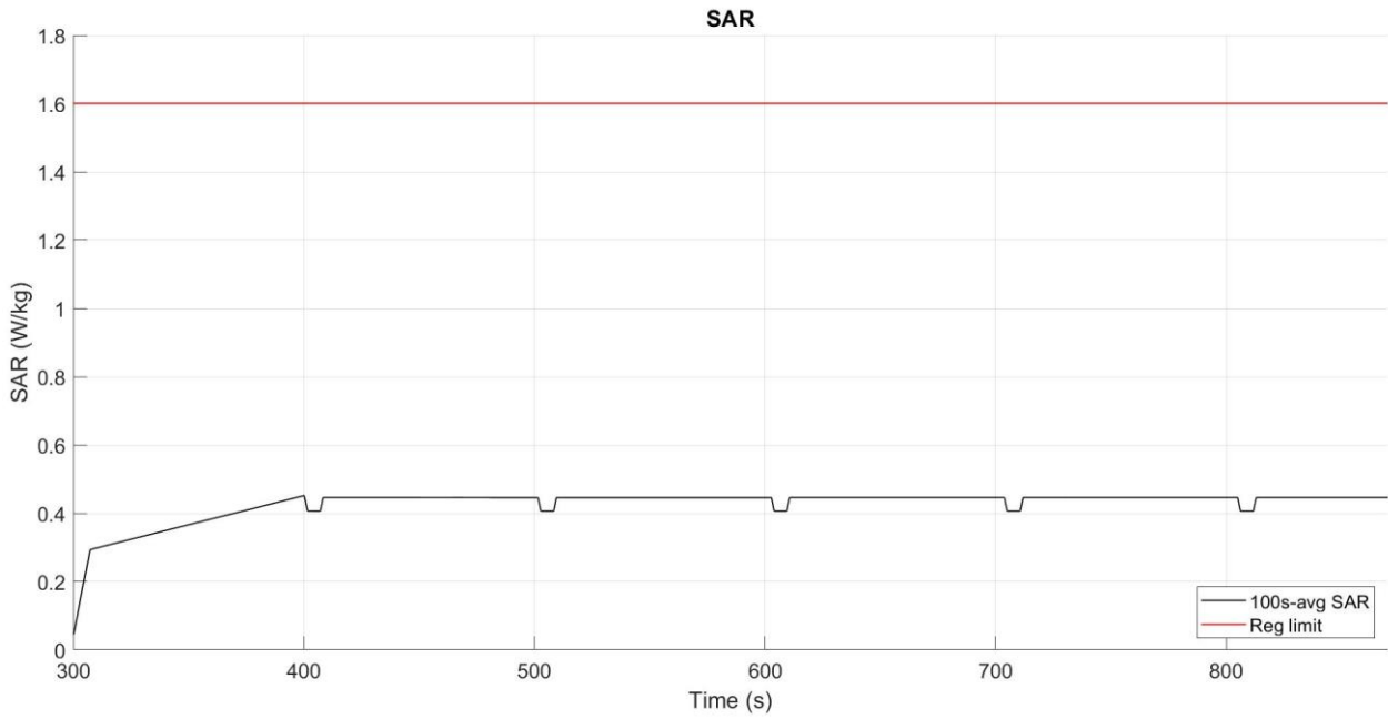
Figure 5- 6 Time-averaged SAR
