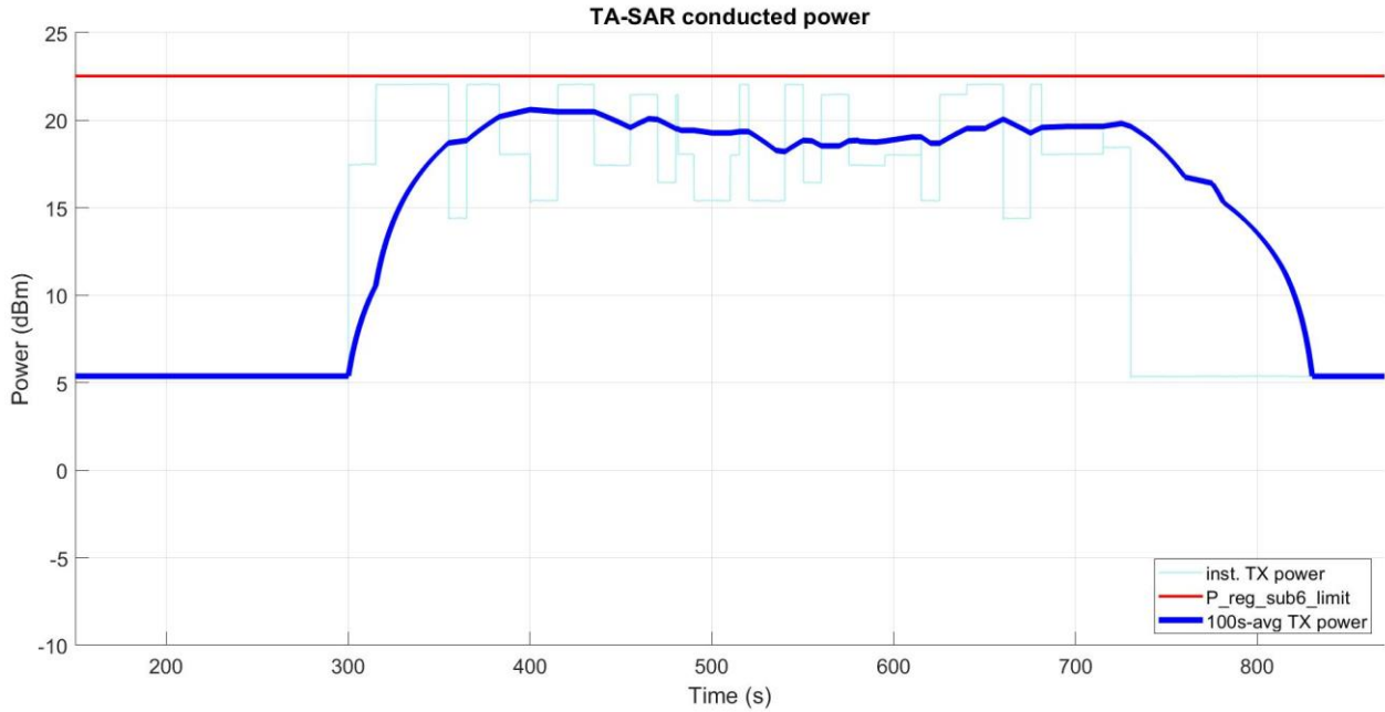
Figure 5- 35 Time-averaged conducted TX power over time
