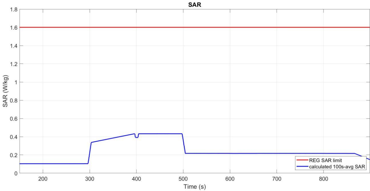
Figure 6-7 Time-averaged SAR
