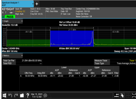
N48(50M)_DFT-s-OFDM_PI_2-BPSK_Edge_1RB_Right_Mid_CH
