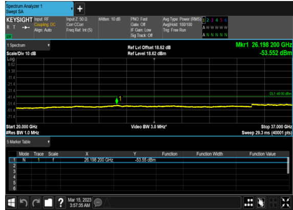
N48(50M)_DFT-s-OFDM_BPSK_Edge_1RB_Left_Low_CH
