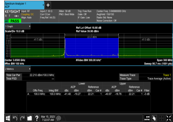
N48(100M)_DFT-s-OFDM_PI_2-BPSK_Edge_1RB_Left_High_CH
