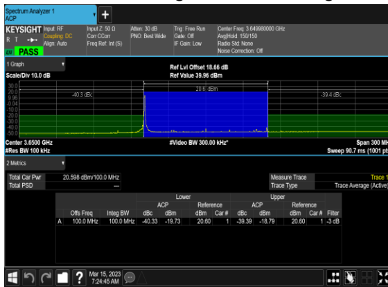
N48(100M)_DFT-s-OFDM_QPSK_Edge_1RB_Left_High_CH
