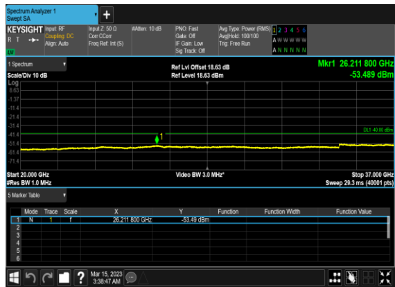
N48(10M)_DFT-s-OFDM_QPSK_Outer_Full_Low_CH
