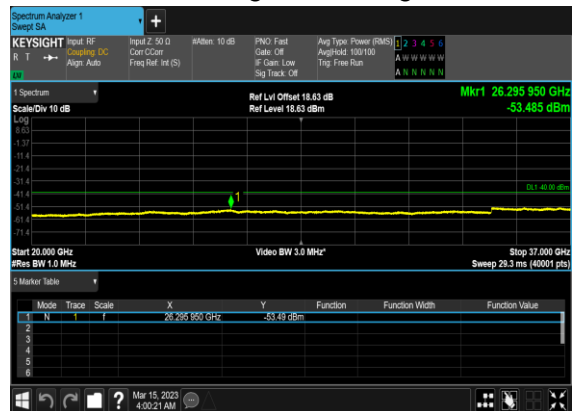
N48(50M)_DFT-s-OFDM_BPSK_Edge_1RB_Right_Low_CH
