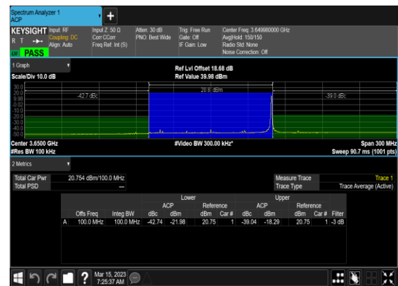
N48(100M)_DFT-s-OFDM_QPSK_Edge_1RB_Right_High_C H
