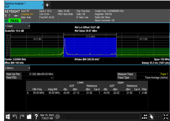
N48(50M)_DFT-s-OFDM_PI_2-BPSK_Edge_1RB_Left_Mid_CH
