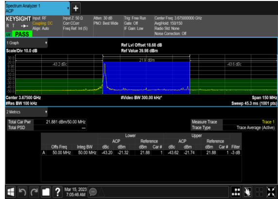
N48(50M)_DFT-s-OFDM_PI_2-BPSK_Edge_1RB_Left_High_CH
