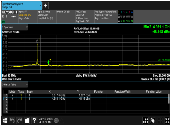
N48(50M)_DFT-s-OFDM_BPSK_Outer_Full_Mid_CH
