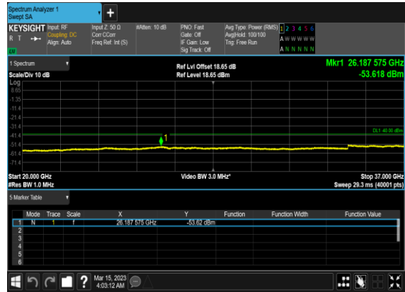
N48(50M)_DFT-s-OFDM_BPSK_Outer_Full_Low_CH
