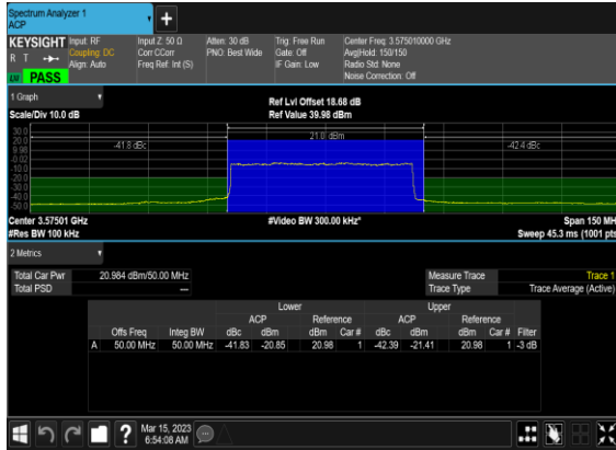
N48(50M)_DFT-s-OFDM_PI_2-BPSK_Outer_Full_Low_CH
