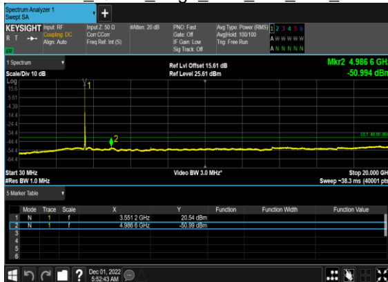
N48(40M)_DFT-s-OFDM_QPSK_Edge_1RB_Left_Low_CH
