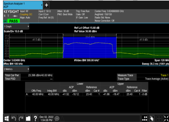
N48(40M)_DFT-s-OFDM_QPSK_Outer_Full_Mid_CH
