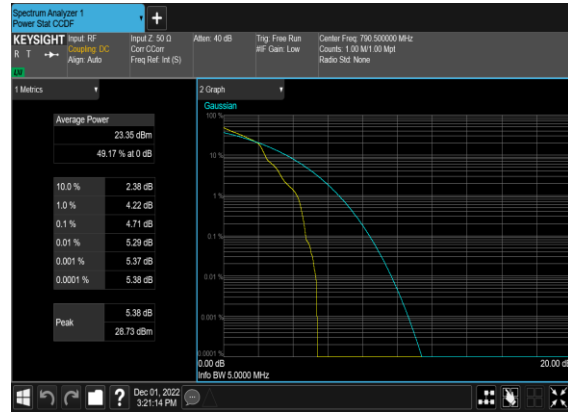
N14(5M)_DFT-s-OFDM_QPSK_Edge_1RB_Left_Low_CH
