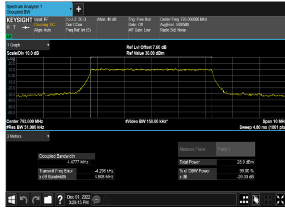
N14(5M)_CP-OFDM_16 QAM_Outer_Full_Mid_CH
