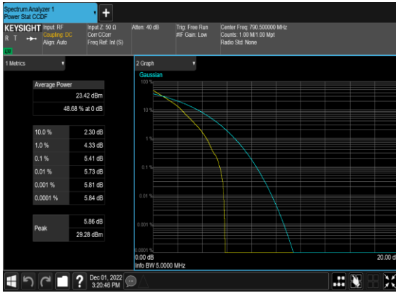
N14(5M)_DFT-s-OFDM_QPSK_Outer_Full_Low_CH
