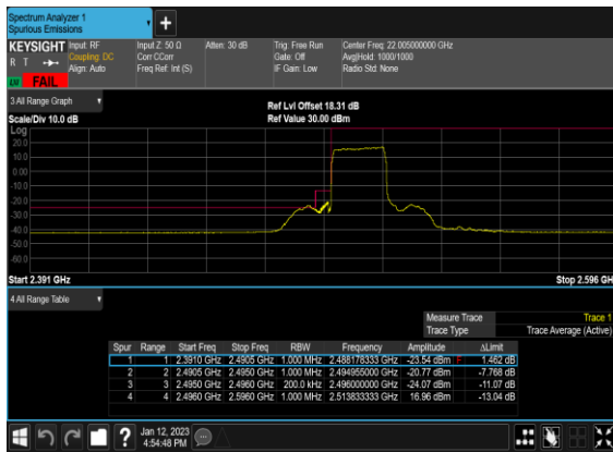
N41(20M)_DFT-s-OFDM_BPSK_Outer_Full_Low_CH
