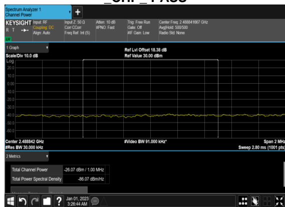
N41(20M)_DFT-s-OFDM_QPSK_Outer_Full_Low_CH CHP_PASS
