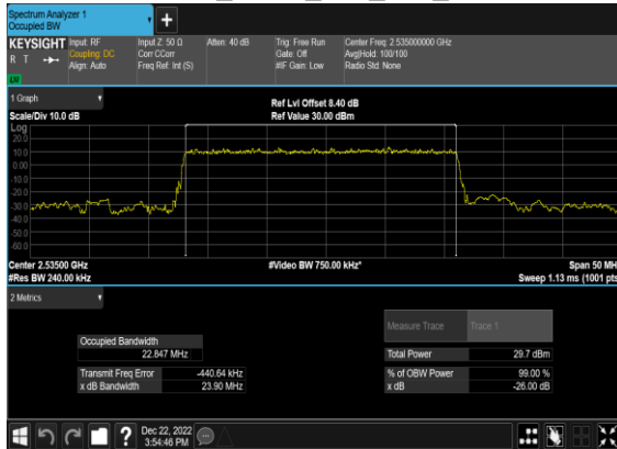
B2_N7(25M)_DFT-s-OFDM_PI_2- BPSK_Outer_Full_Mid_CH
