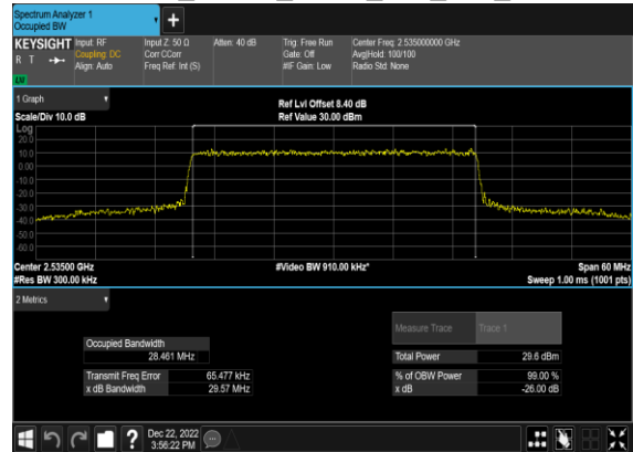
B2_N7(30M)_DFT-s- OFDM_QPSK_Outer_Full_Mid_CH
