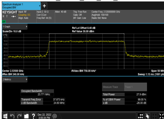
B2_N7(25M)_CP-OFDM_64 QAM_Outer_Full_Mid_CH
