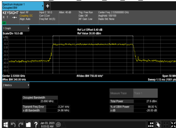
B2_N7(25M)_CP- OFDM_QPSK_Outer_Full_Mid_CH
