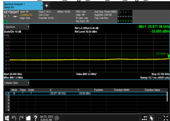
B2_N7(40M)_DFT-s-OFDM_BPSK_Edge_1RB_Left_High_CH
