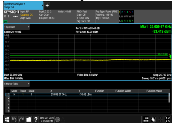
B2_N7(40M)_DFT-s-OFDM_QPSK_Edge_1RB_Left_Mid_CH
