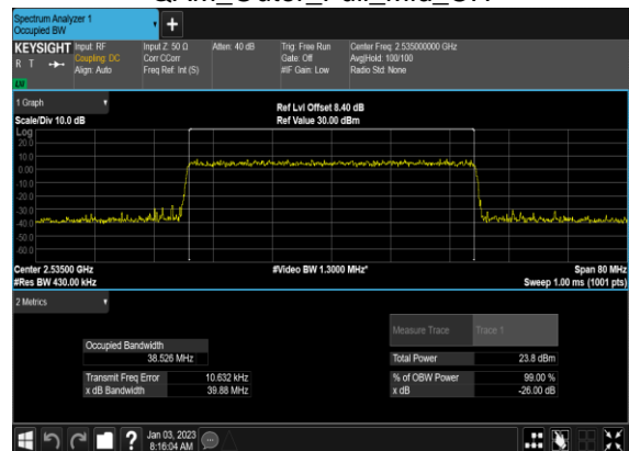
B2_N7(40M)_CP-OFDM_256 QAM_Outer_Full_Mid_CH
