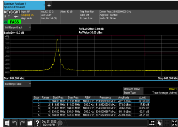
N26(20M)_DFT-s-OFDM_BPSK_Edge_1RB_Left_Mid_CH
