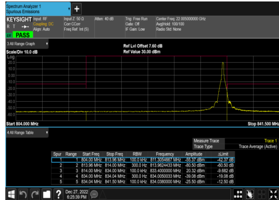
N26(20M)_DFT-s-OFDM_BPSK_Edge_1RB_Right_Mid_CH
