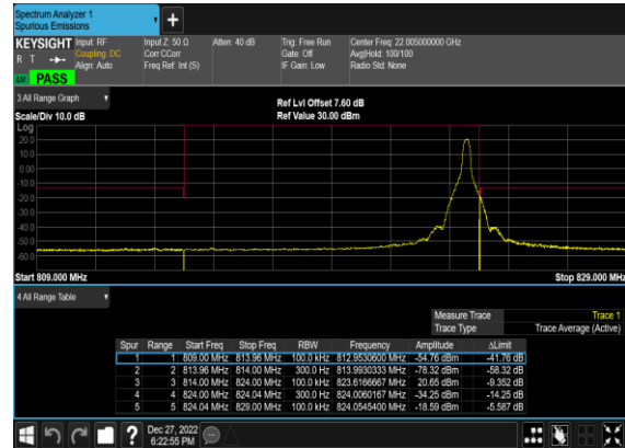
N26(10M)_DFT-s- OFDM_BPSK_Edge_1RB_Right_Mid_CH
