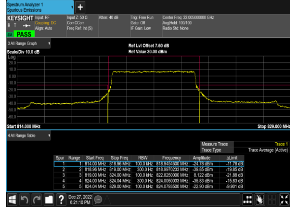
N26(5M)_DFT-s- OFDM_BPSK_Outer_Full_High_CH
