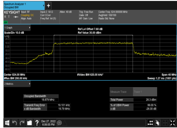
N26(20M)_CP-OFDM_16 QAM_Outer_Full_Mid_CH
