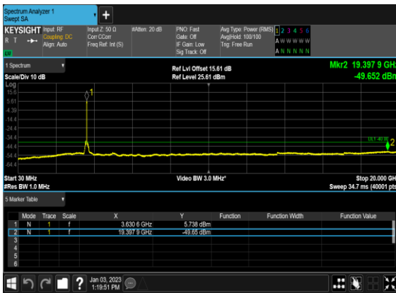
N48(40M)_DFT-s-OFDM_QPSK_Outer_Full_Mid_CH
