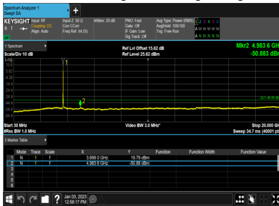
N48(20M)_DFT-s-OFDM_BPSK_Edge_1RB_Right_High_CH
