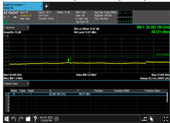
N48(40M)_DFT-s-OFDM_BPSK_Edge_1RB_Right_High_CH
