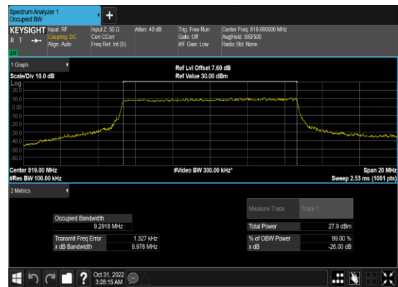
N26(10M)_CP-OFDM_16 QAM_Outer_Full_Mid_CH
