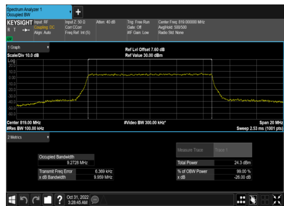
N26(10M)_CP-OFDM_256 QAM_Outer_Full_Mid_CH
