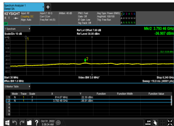
N26(20M)_DFT-s-OFDM_QPSK_Edge_1RB_Left_Mi
