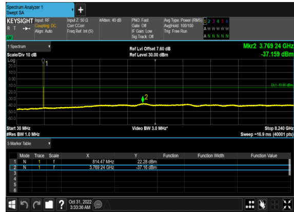
N26(5M)_DFT-s-OFDM_QPSK_Edge_1RB_Left_Mid
