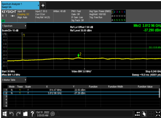
N26(5M)_DFT-s-OFDM_BPSK_Edge_1RB_Left_Mid
