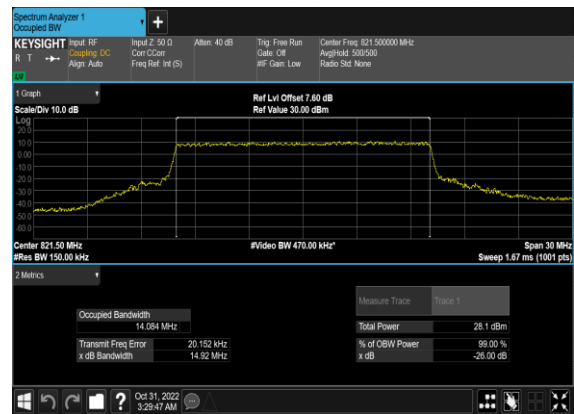
N26(15M)_CP-OFDM_16 QAM_Outer_Full_Mid_CH
