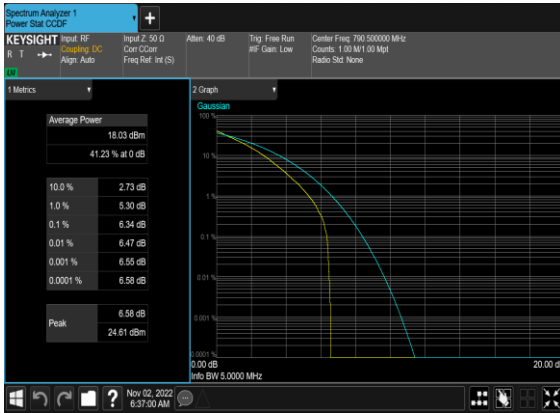
N14(5M)_DFT-s-OFDM_QPSK_Outer_Full_Low_CH
