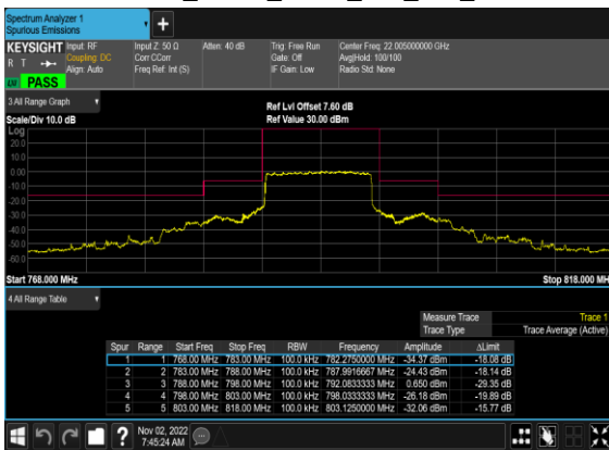
N14(10M)_DFT-s- OFDM_BPSK_Outer_Full_Mid_CH
