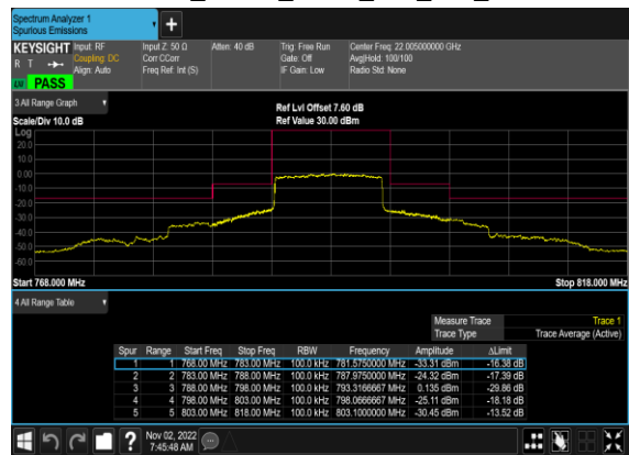
N14(10M)_DFT-s- OFDM_QPSK_Outer_Full_Mid_CH
