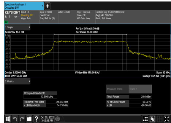
N77(15M)_CP-OFDM_16 QAM_Outer_Full_Mid_CH
