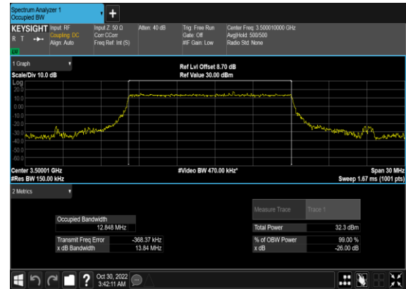
N77(15M)_DFT-s- OFDM_QPSK_Outer_Full_Mid_CH
