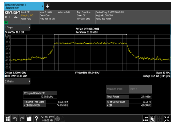
N77(15M)_CP-OFDM_256 QAM_Outer_Full_Mid_CH
