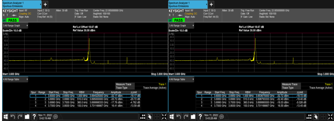
N77(50M)_DFT-s- OFDM_BPSK_Edge_1RB_Left_Low_CH
