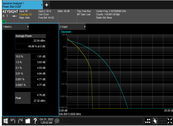
N30(5M)_DFT-s-OFDM_PI_2-BPSK_Outer_Full_L ow_CH
