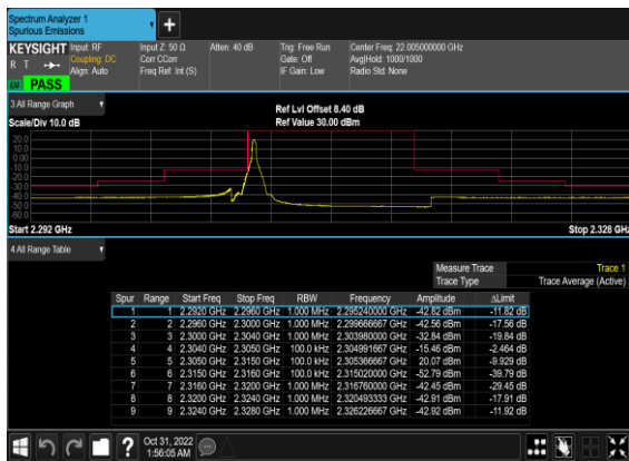
N30(10M)_DFT-s-OFDM_BPSK_Edge_1RB_Right_
