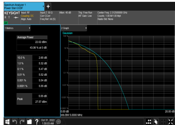
N30(5M)_DFT-s-OFDM_QPSK_Edge_1RB_Left_High_
