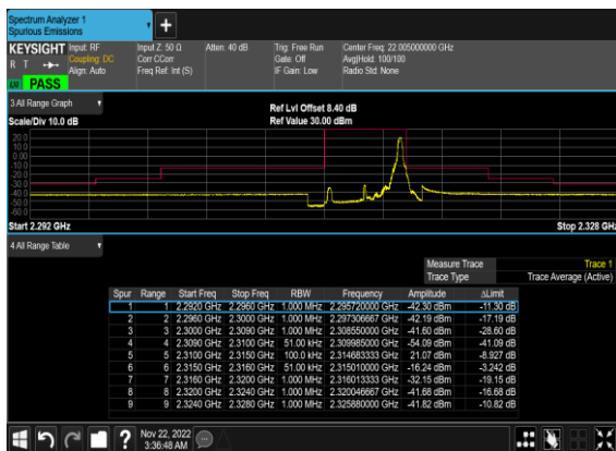
N30(5M)_DFT-s-OFDM_BPSK_Edge_1RB_Right_Hi
