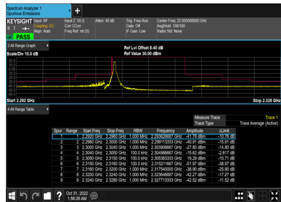
N30(10M)_DFT-s-OFDM_QPSK_Edge_1RB_Right_
