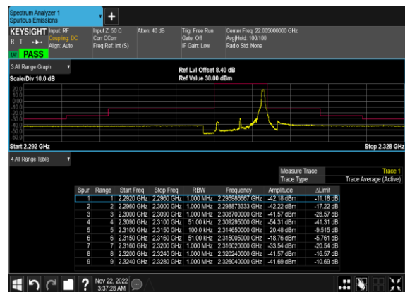
N30(5M)_DFT-s-OFDM_QPSK_Edge_1RB_Right_Hi
