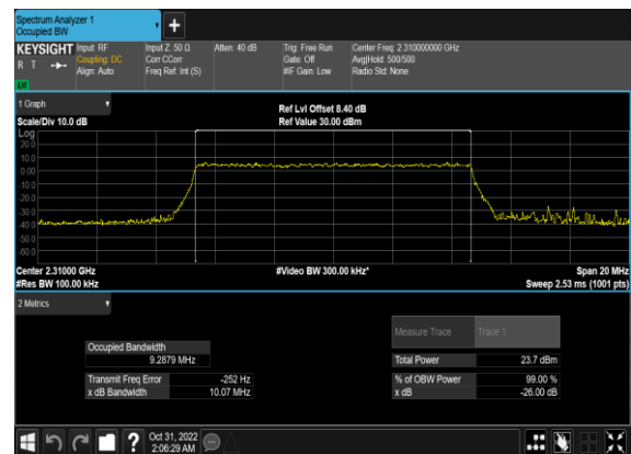
N30(10M)_CP-OFDM_256 QAM_Outer_Full_Low_CH
