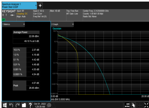
N30(5M)_DFT-s-OFDM_QPSK_Outer_Full_High_
