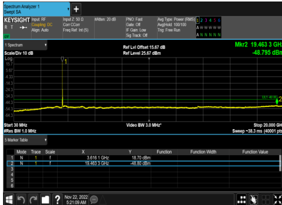
N48(20M)_DFT-s-OFDM_BPSK_Edge_1RB_Left_Mid_CH
