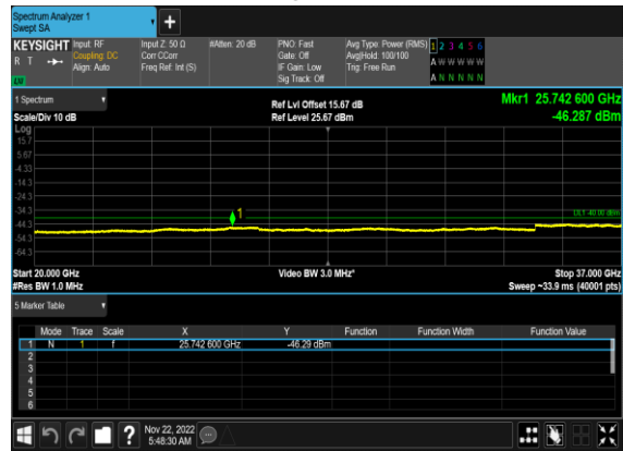
N48(40M)_DFT-s-OFDM_QPSK_Edge_1RB_Left_Mid_CH
