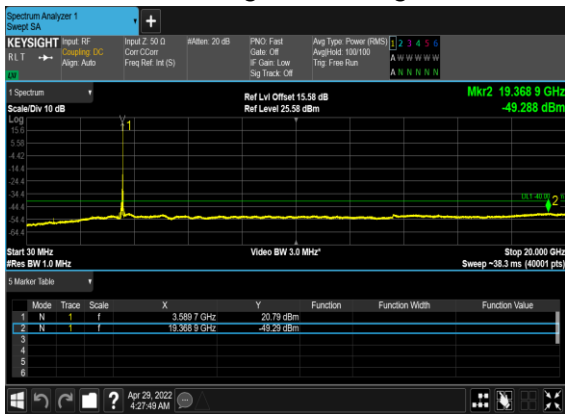
N48(40M)_DFT-s-OFDM_BPSK_Edge_1RB_Right_Low_CH
