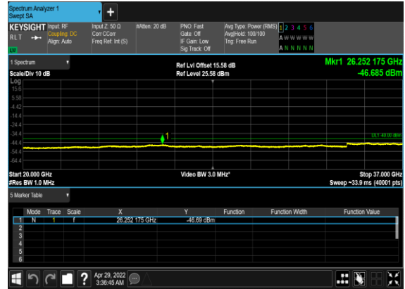
N48(10M)_DFT-s-OFDM_BPSK_Edge_1RB_Left_Low_CH
