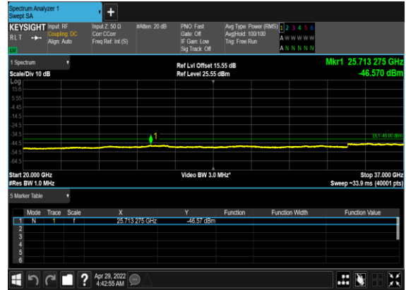
N48(40M)_DFT-s-OFDM_BPSK_Edge_1RB_Left_High_CH
