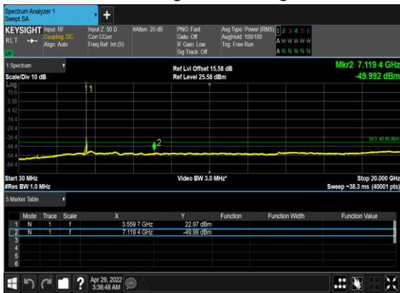
N48(10M)_DFT-s-OFDM_BPSK_Edge_1RB_Right_Low_CH
