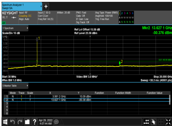
N48(20M)_DFT-s- OFDM_QPSK_Outer_Full_Low_CH
