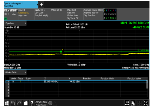
N48(20M)_DFT-s-OFDM_BPSK_Outer_Full_High_CH
