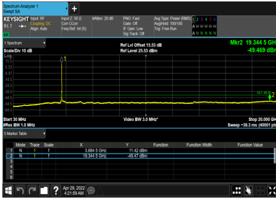
N48(20M)_DFT-s-OFDM_BPSK_Outer_Full_High_CH
