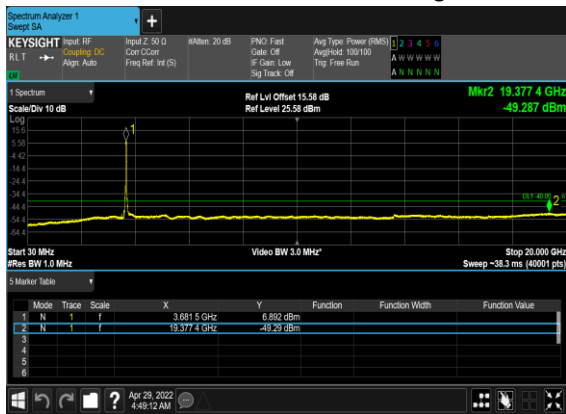
N48(40M)_DFT-s- OFDM_QPSK_Outer_Full_High_CH
