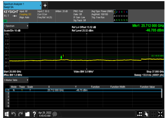
N48(40M)_DFT-s-OFDM_BPSK_Edge_1RB_Right_High_CH
