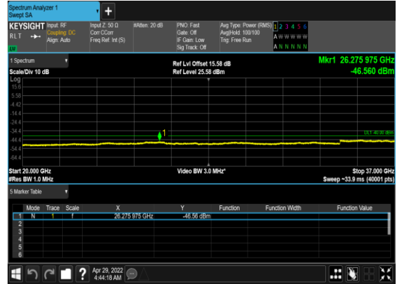
N48(40M)_DFT-s-OFDM_QPSK_Edge_1RB_Left_High_CH
