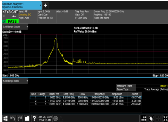
B66_N2(20M)_DFT-s-OFDM_BPSK_Edge_1RB_Right_High_CH
