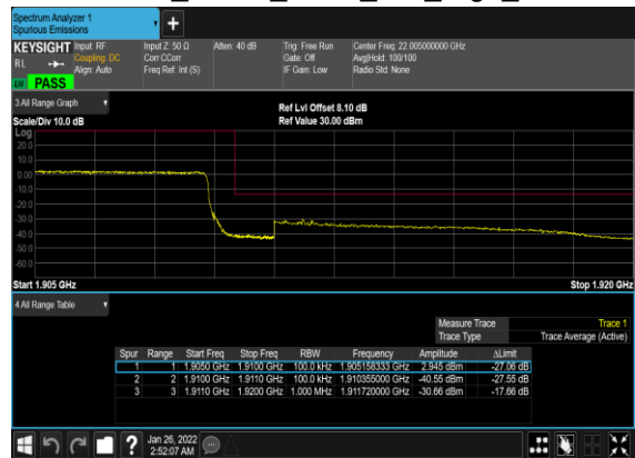
B66_N2(10M)_DFT-s-OFDM_QPSK_Outer_Full_High_CH
