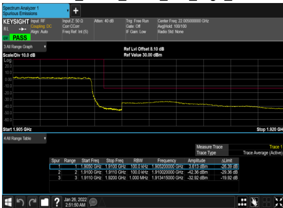
B66_N2(10M)_DFT-s-OFDM_BPSK_Outer_Full_High_CH
