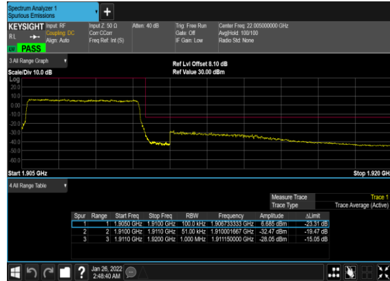
B66_N2(5M)_DFT-s-OFDM_QPSK_Outer_Full_High_CH
