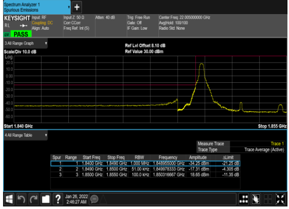
B66_N2(5M)_DFT-s-OFDM_QPSK_Edge_1RB_Left_Low_CH
