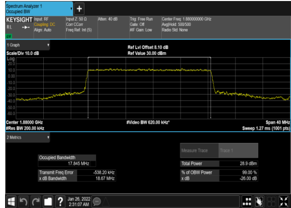
B66_N2(20M)_DFT-s- OFDM_QPSK_Outer_Full_Mid_CH
