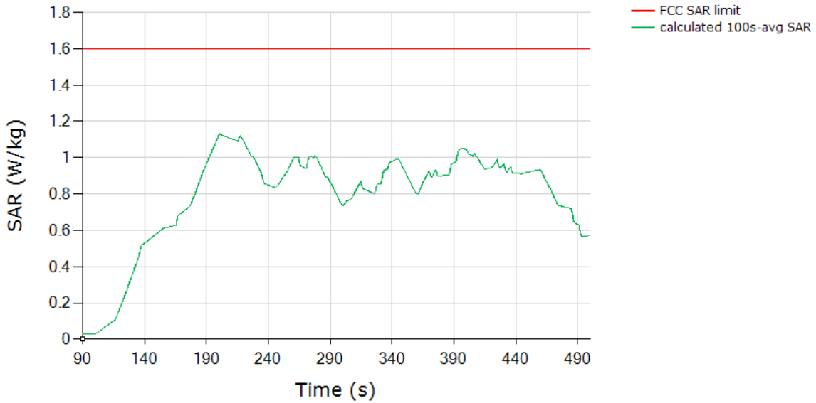
SAR (Test Sequence 2) Tech: 5GNR, Band n77
