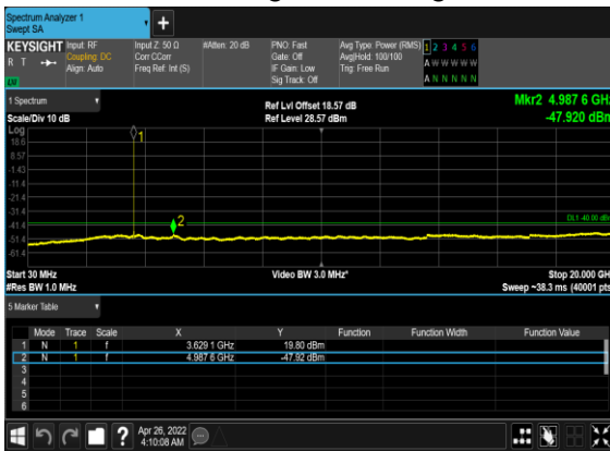
N48(10M)_DFT-s-OFDM_BPSK_Edge_1RB_Right_Mid_CH
