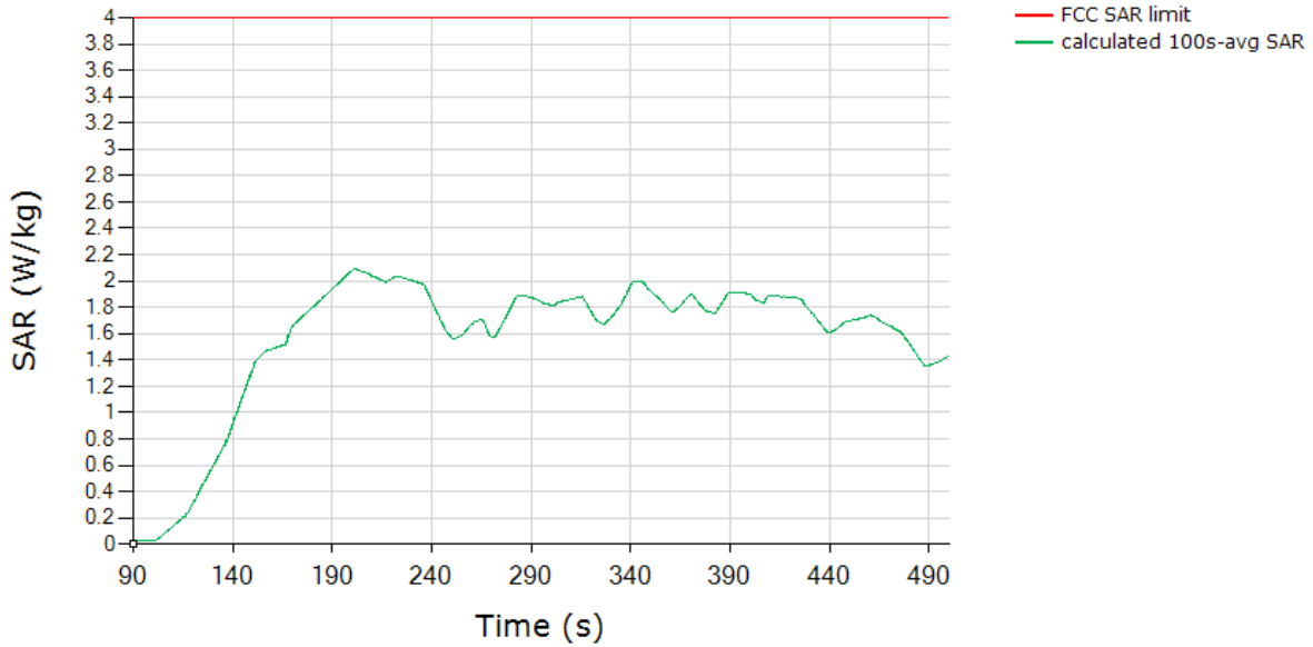
SAR (Test Sequence 2) Tech: 5G NR, Band 2
