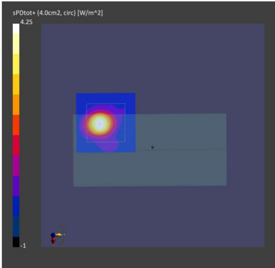
Figure 8-4: 4cm2-averaged power density distribution measured at input.power.limit of 4.25dBm on the back surface for n261 beam 41
