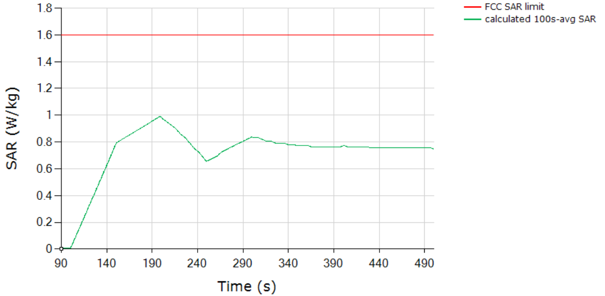
SAR (Test Sequence 1) Tech: GSM, Band 1900
