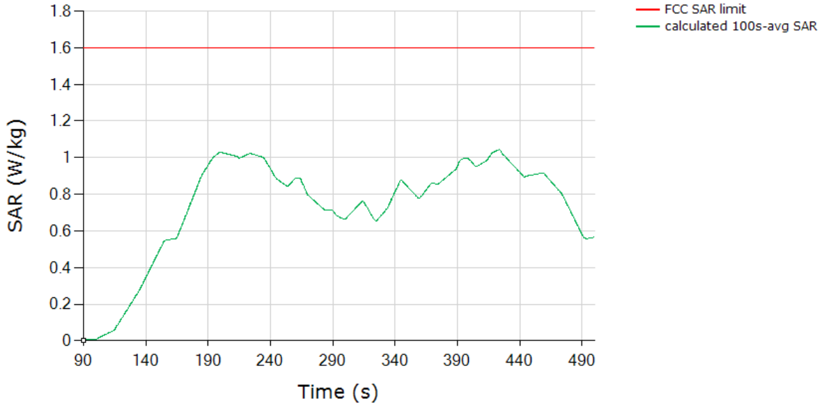
SAR (Test Sequence 2) Tech: WCDMA, Band 5
