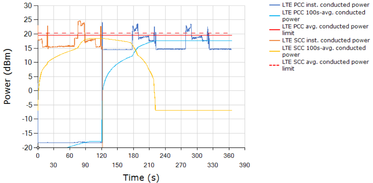
LTE PCC/SCC Instantaneous and Time-averaged TX Power Tech: LTE, Band 2 / Tech: LTE, Band 66
