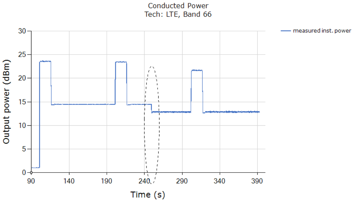
Plot Notes: The conducted power plot shows expected Tx transition.
