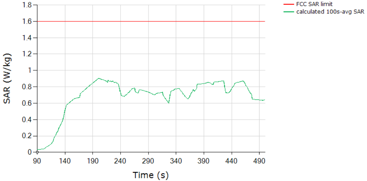
SAR (Test Sequence 2) Tech: 5GNR, Band 66
