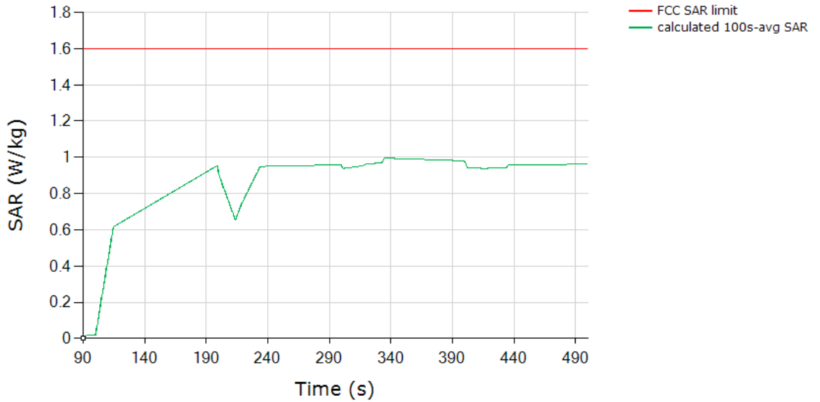
SAR (Test Sequence 1) Tech: LTE, Band 66
