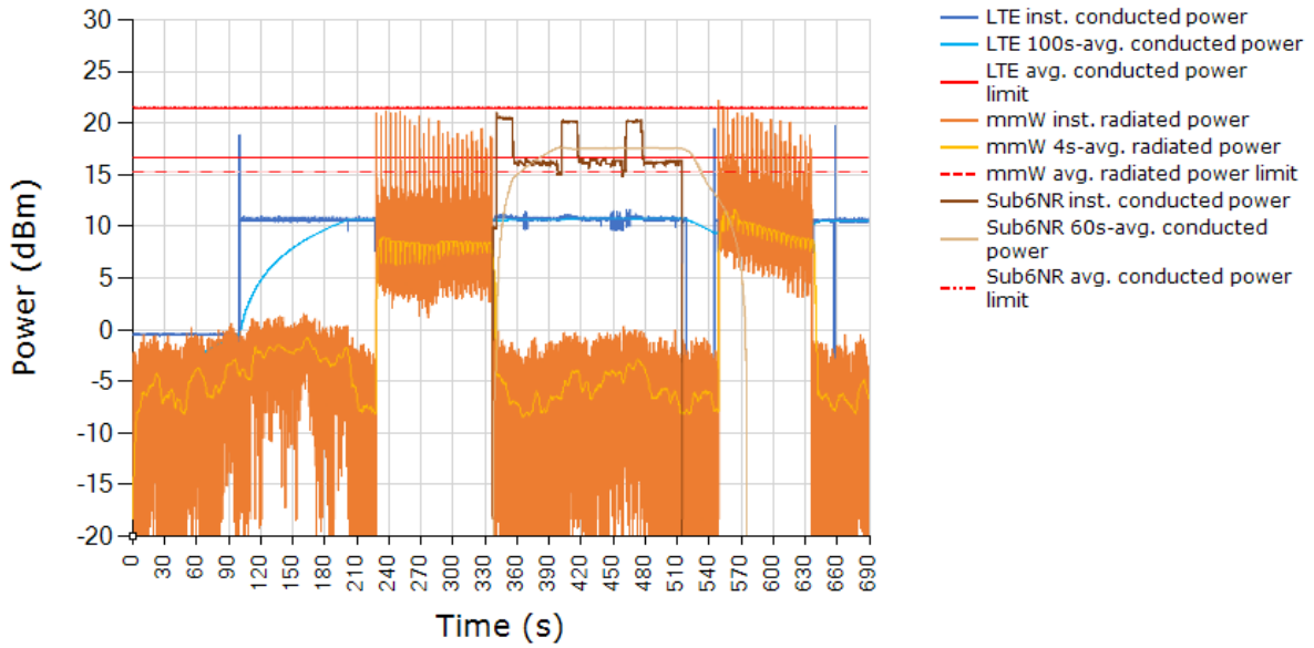
LTE and mmW Instantaneous and Time-averaged TX Power Tech: LTE, Band 2 / Tech: NR5G SUB6, Band n77
