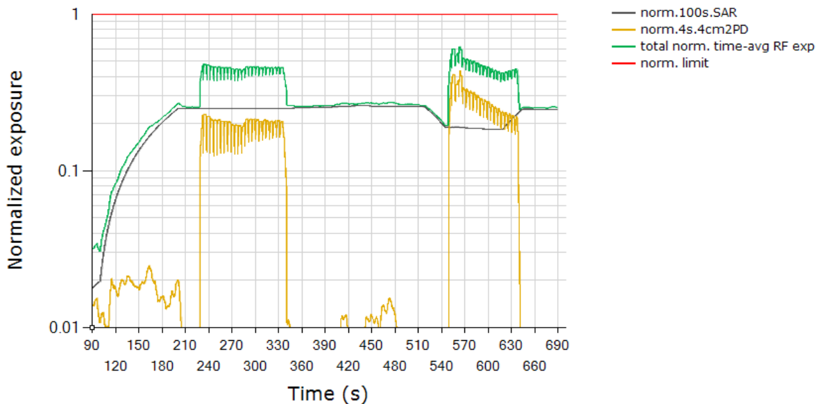
Total LTE + FR2 Normalized Time-averaged RF Exposure Tech: LTE, Band 2 / Tech: NR5G MMW, Band n261
