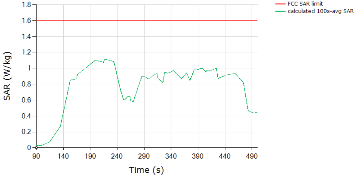
SAR (Test Sequence 2) Tech: LTE, Band 2
