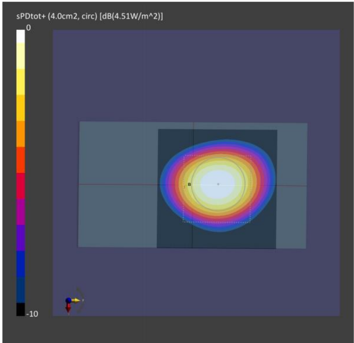
Figure 8-4: 4cm2-averaged power density distribution measured at input.power.limit of 4.51dBm on the back surface for n261 beam 40
