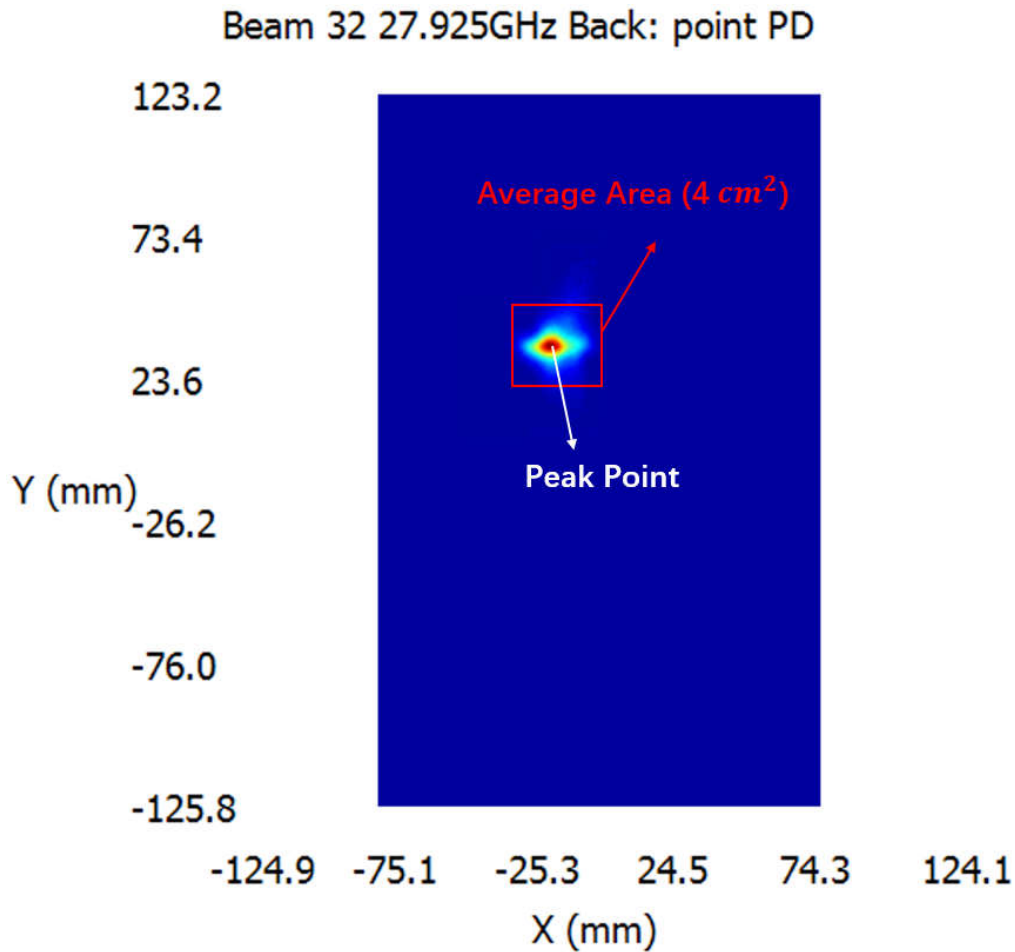
Figure 2.4.1-1 Power density distribution (Example)
