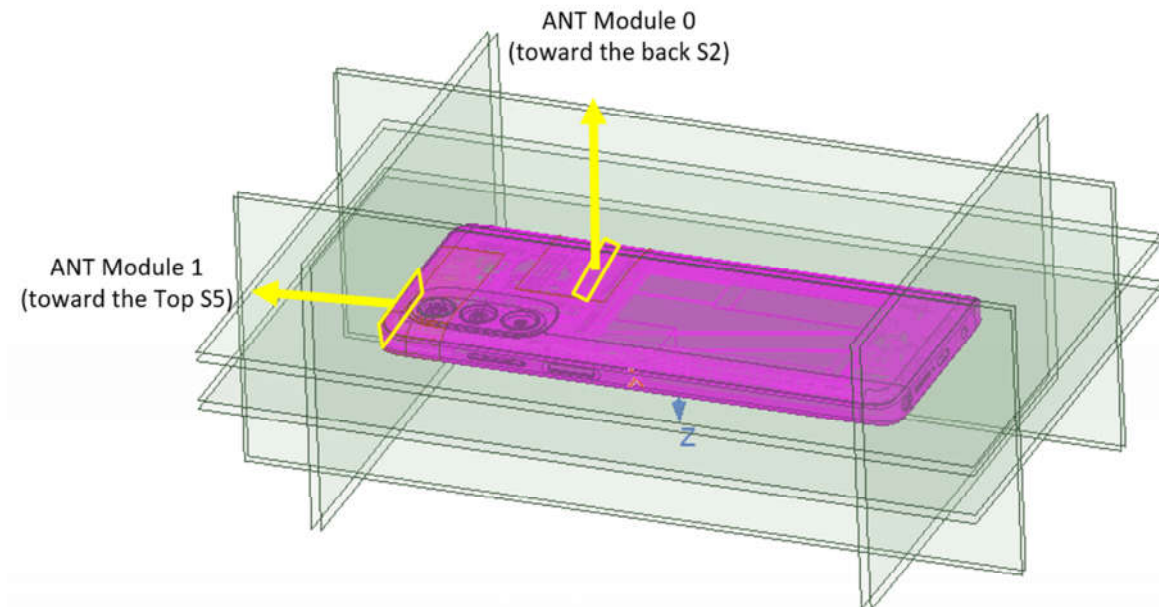
Figure 2.3.5-1: PD surface(2mm&5mm)
