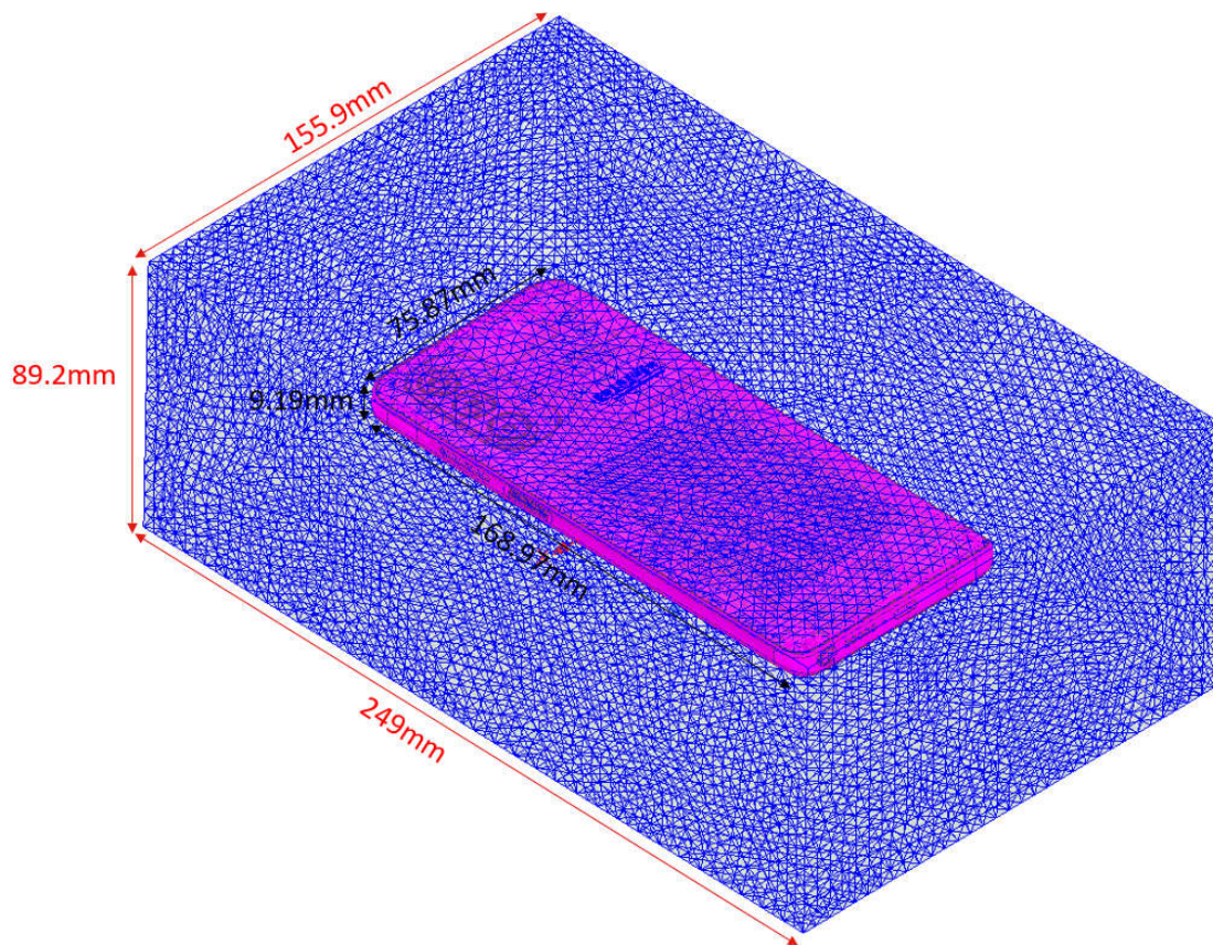
Figure 2.3.3-1: Example of the adaptive mesh technique & Mobile size
