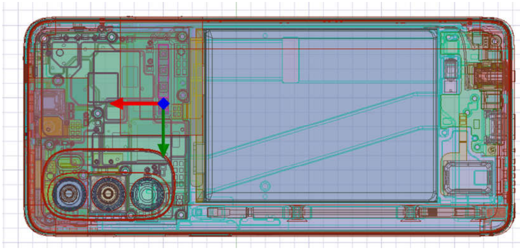
Figure 2.3.4-1: 3D model used for Module 0 ( Back module ), the antenna array is highlighted
