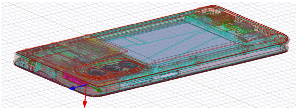
Figure 2.3.4-1: 3D model used for Module 1 ( Top module ), the antenna array is highlighted
