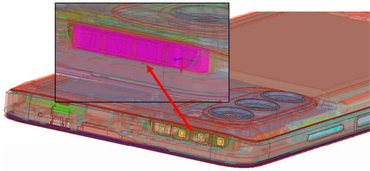
Figure 2.3.7.1 mmWave module 1
