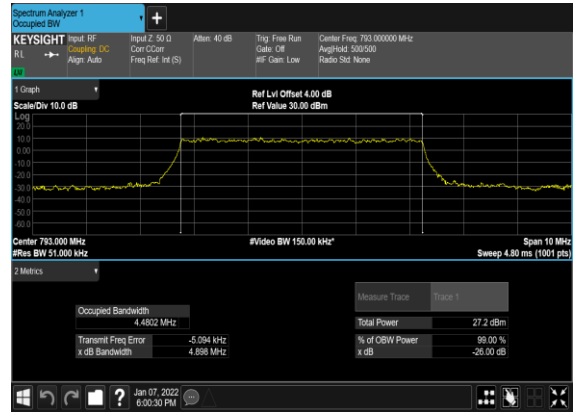
N14(5M)_CP-OFDM_16 QAM_Outer_Full_Mid_CH
