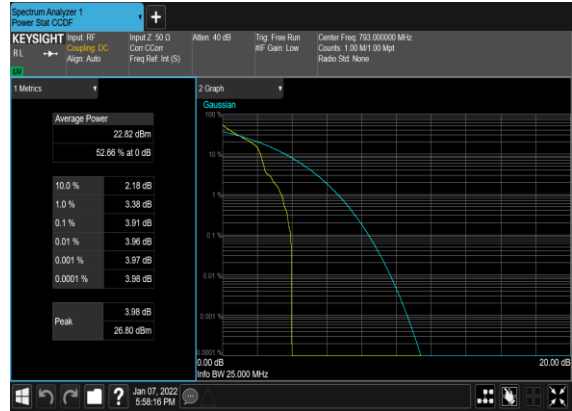
N14(10M)_DFT-s-OFDM_PI_2-BPSK_Edge_1RB_Left_Mid_CH
