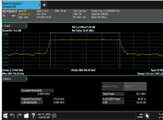
B2_N30(10M)_DFT-s-OFDM_PI_2- BPSK_Outer_Full_Low_CH
