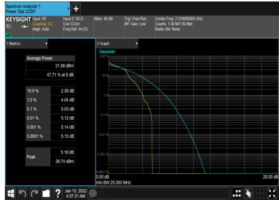
B2_N30(10M)_DFT-s-OFDM_QPSK_Edge_1RB_Left_Low_CH
