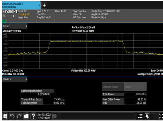
B2_N30(10M)_CP- OFDM_QPSK_Outer_Full_Low_CH
