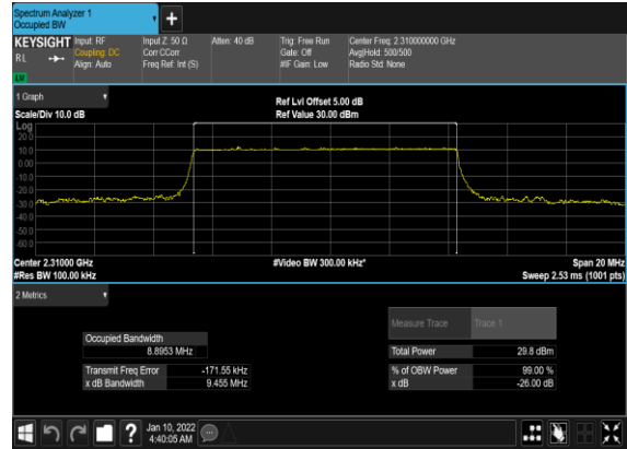
B2_N30(10M)_DFT-s- OFDM_QPSK_Outer_Full_Low_CH
