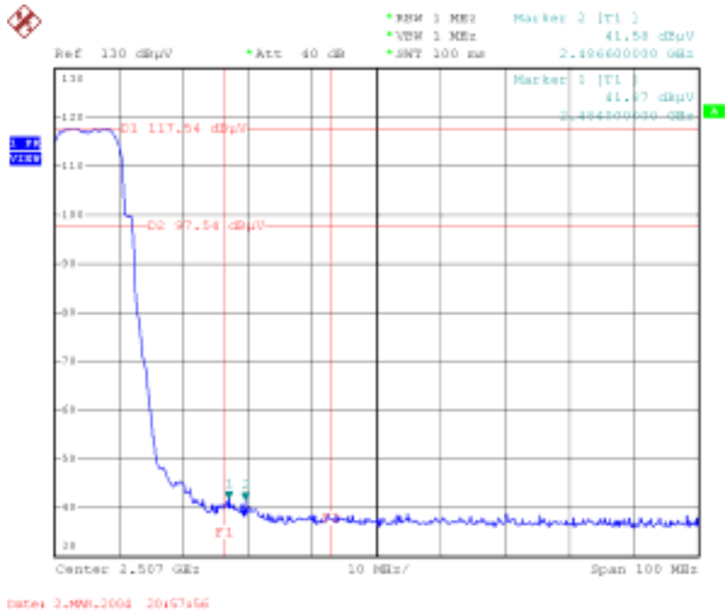
Higher Band Edge (Peak)
