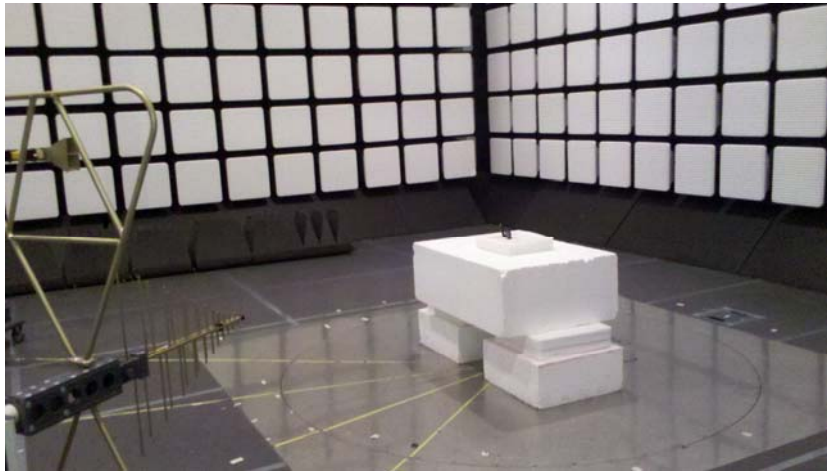
Radiated Emissions
